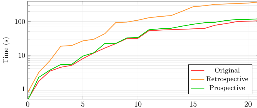
Fig. 5: Quantile plot of execution times for the isolated implementation
