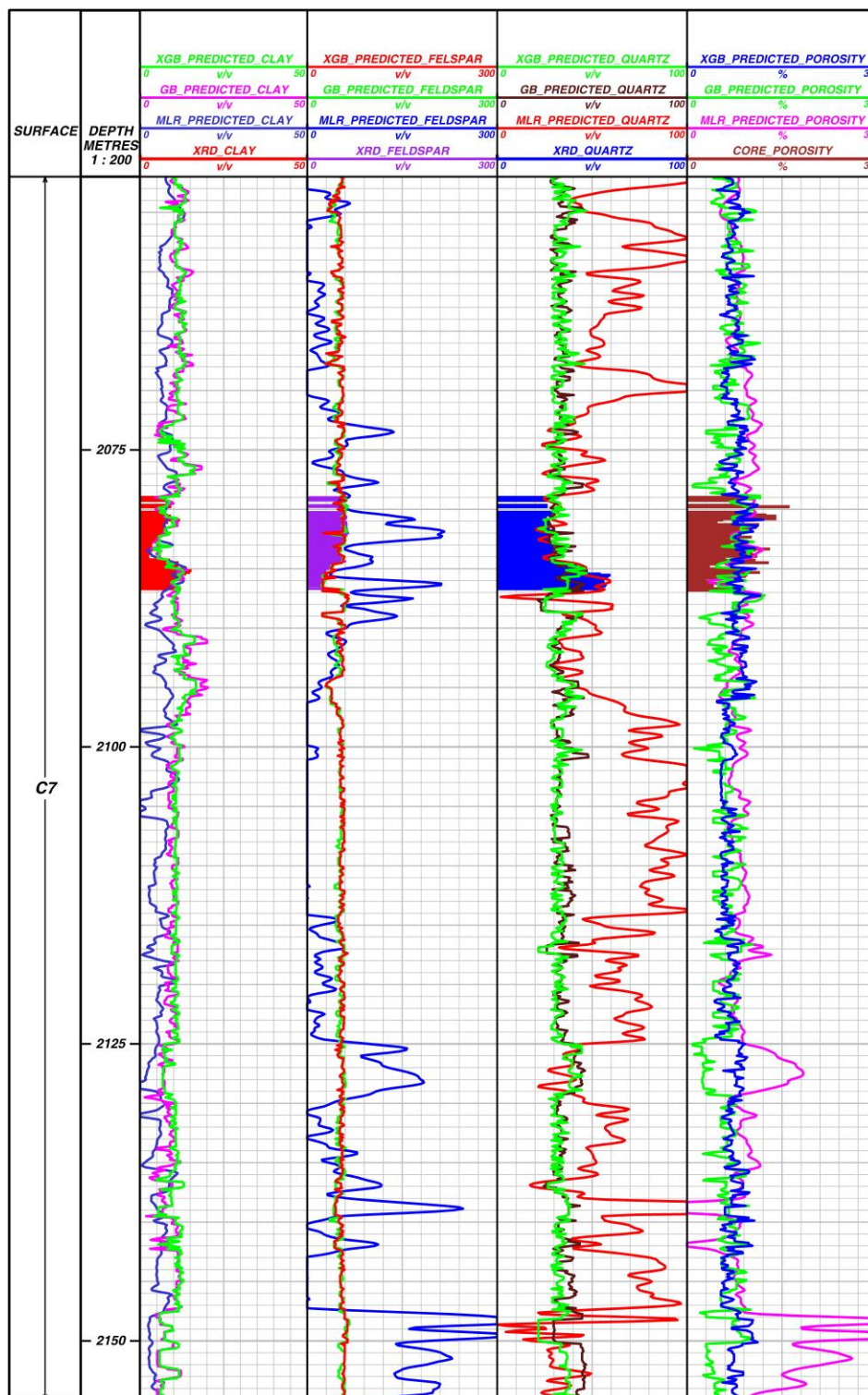
Fig. 5.11: XRD analysis for estimating the mineral composition and core porosity (in red, purple, blue, and magenta curves) and the curve of predicted mineral composition using MLR, Gradient Boost, and XGBoost method in Well 1.
