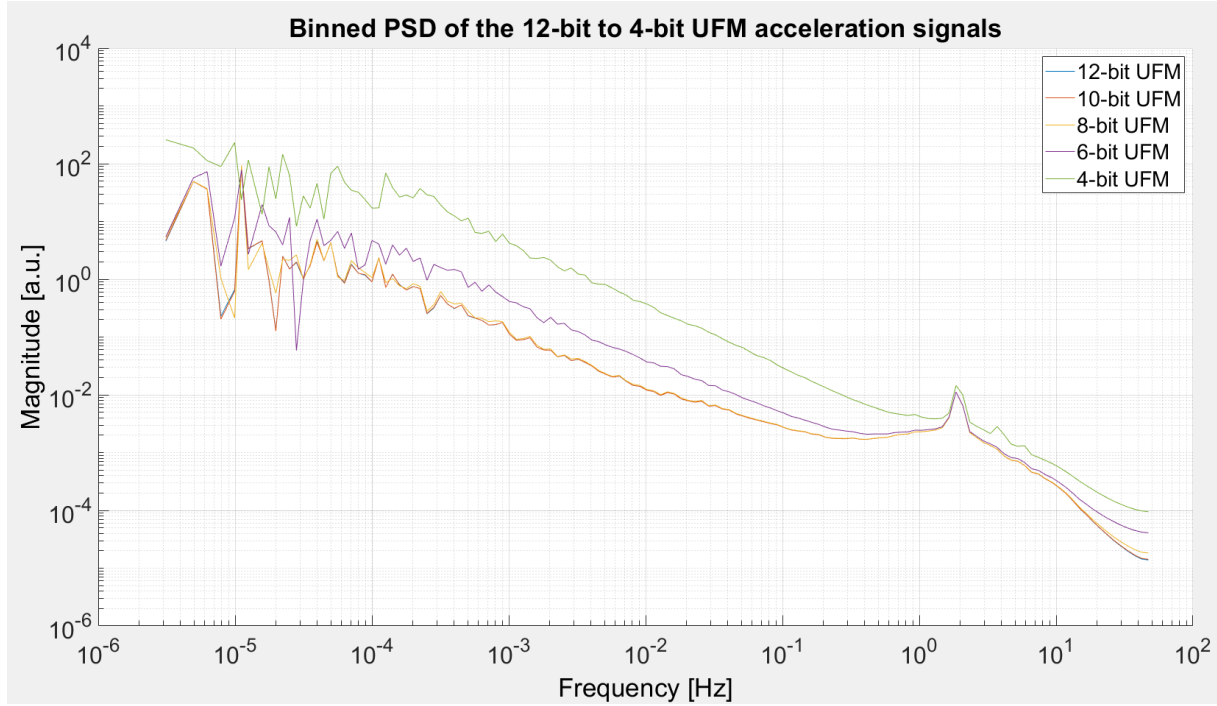
Figure 4.7: The binned power spectral density of the 12-bit (blue), 10-bit (red), 8-bit (yellow), 6-bit (purple) and 4-bit (green) versions of the same UFM acceleration
