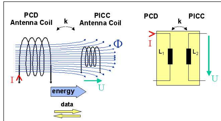
Figure 2: Transformer Model
