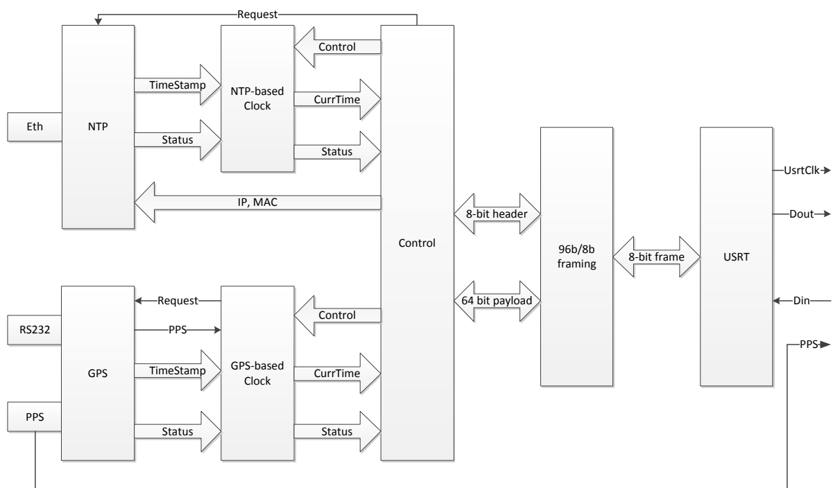
WCLOCK architecture
