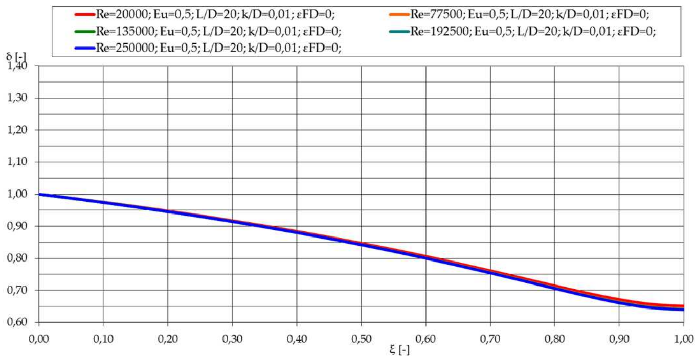
7.12. diagram: A dimensionless diameter change as a function of dimensionless length.
