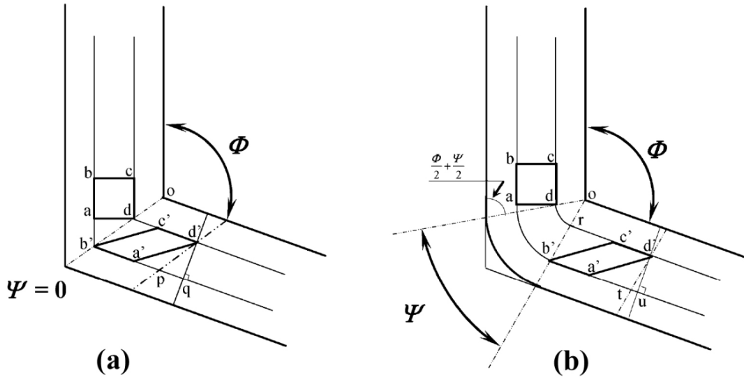
Fig. 1.2 Shear deformation during ECAP: a) \Psi = 0 or b) \Psi \neq 0 [22]
