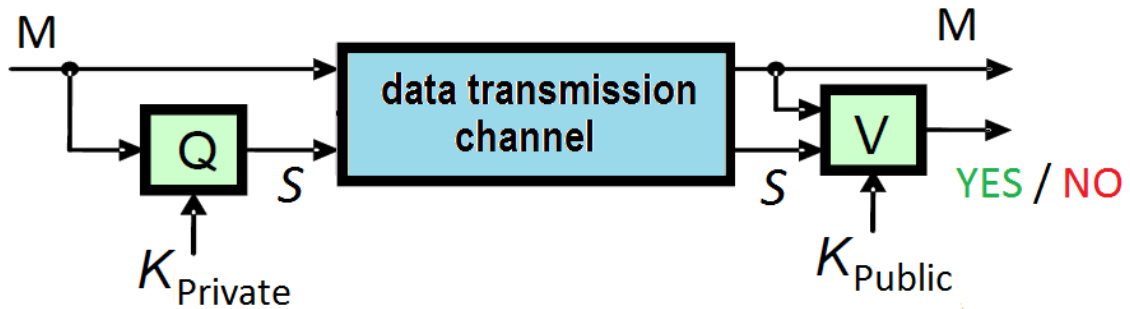
Figure 7.2: Block diagram of the cryptosystem for message authentication
