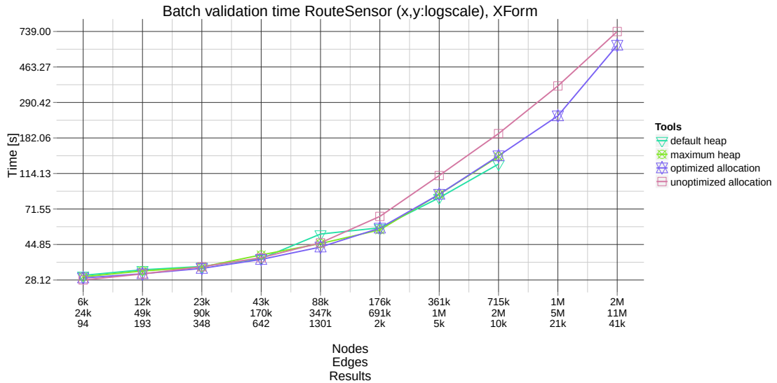
Figure 6.1. Runtime of the read and first check phases on a slow (10 Mbit) network.
