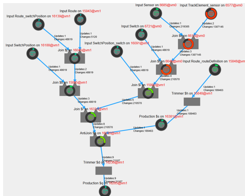
Figure 6.4. RouteSensor measurement Rete network monitoring.
