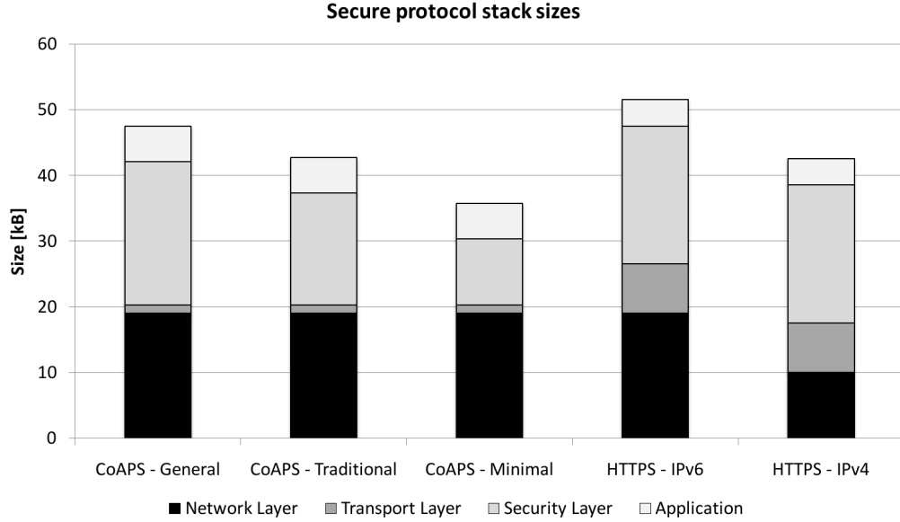
Figure 4.2: Stack code size summary for TCP and UDP bound application layer protocols.
