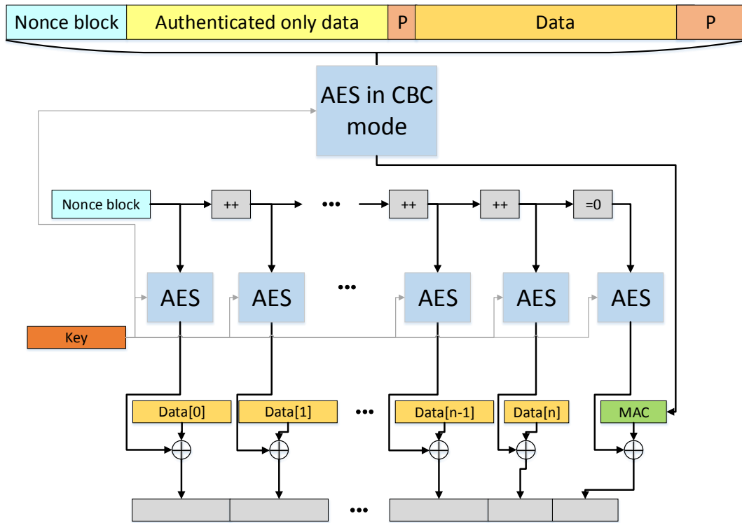
Figure 2.8: (D)TLS AES in CCM mode – authenticated encryption
