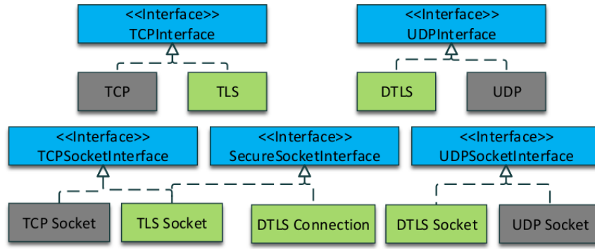
Figure 3.1: Interfaces for the sockets and transport layers
