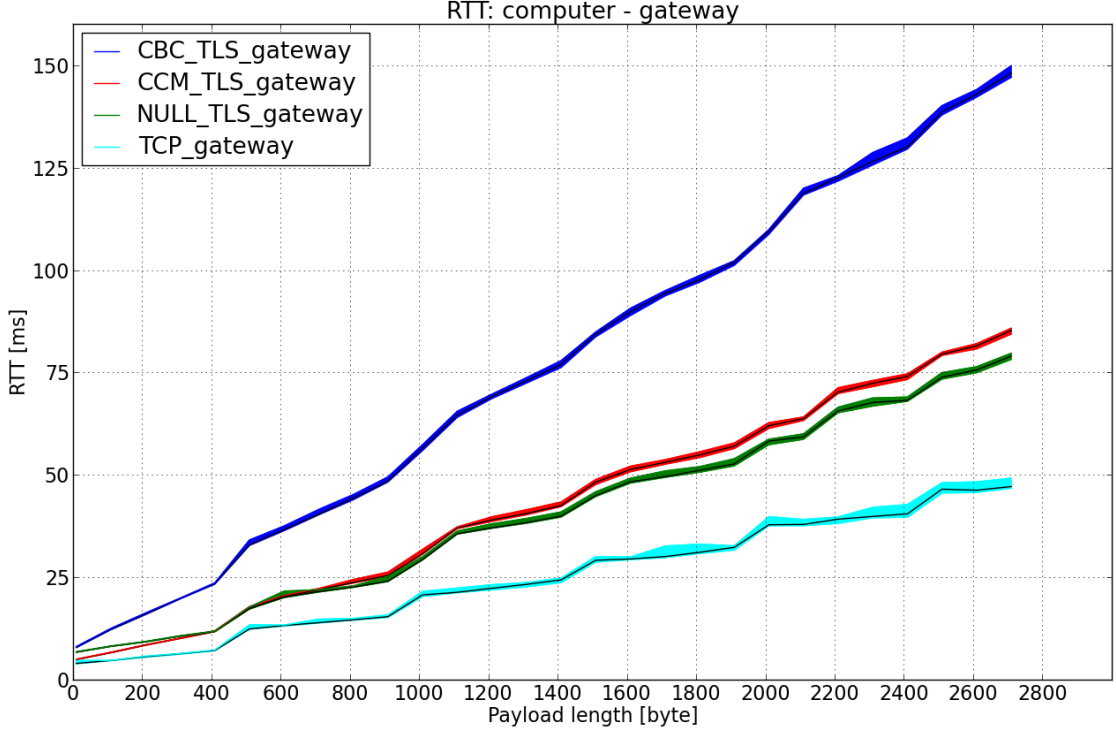
Figure 4.6: TCP/TLS round-trip-times for the Computer-Gateway-Scenario
