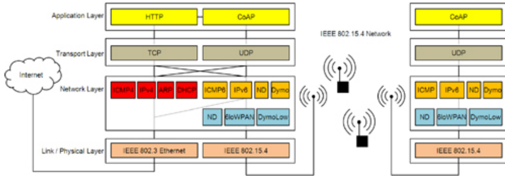
Figure 1.2: iSense IPv4 and IPv6 Dual Network Stack (Source: www.coalesenses.com )
