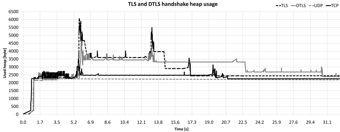
Figure 4.3: Heap usage for TLS/DTLS (and TCP/UDP for reference).
