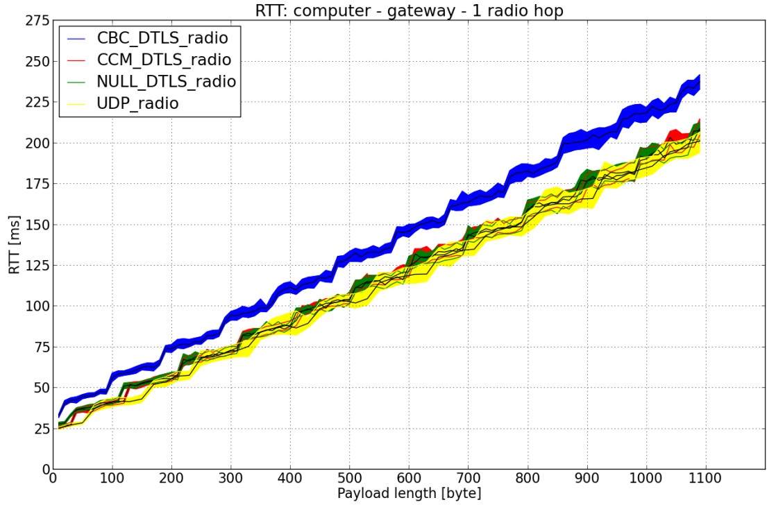
Figure 4.8: Round-trip-times for the Computer-Gateway-1 radio hop-Scenario
