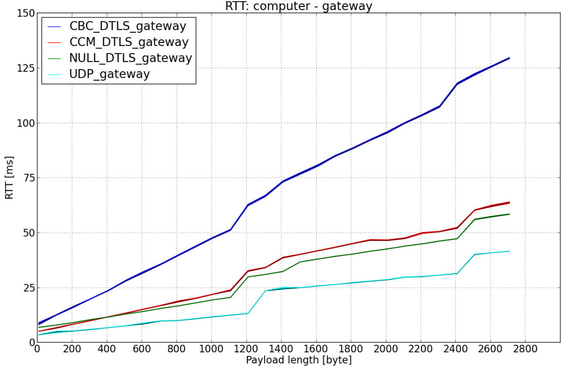
Figure 4.7: UDP/DTLS round-trip-times for the Computer-Gateway-Scenario
