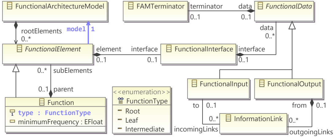
Figure 5.2: Metamodel for functional architecture of avionics systems
