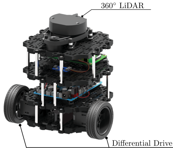
Figure 1: ROBOTIS' TurtleBot3 Burger platform, with a mounted 360° LiDAR on top, and a differential drive (image source: www.robosklep.com ).
