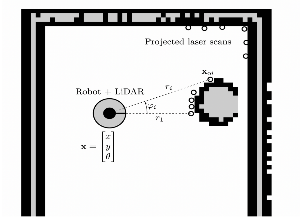
Figure 8: Projection of the LiDAR scans to the OGM, based on the pose of the robot.
