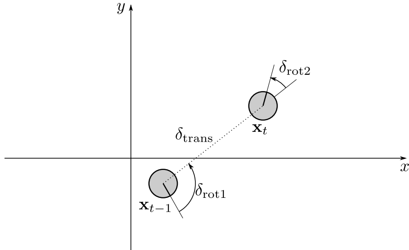
Figure 4: Rotation-translation-rotation transition sequence from state \mathbf{x}_{t-1} to \mathbf{x}_t .
