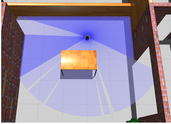
Figure 2: Visualized 2D LiDAR measurement of the TurtleBot3 in a house environment, using the Gazebo simulator.
