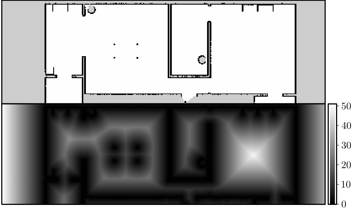
Figure 7: Part of the OGM of the TurtleBot3 House, and its distance transform.
