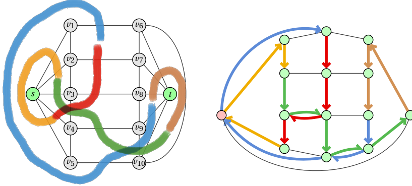
(a) The network topology and the SRLGs ( \mathcal{S}_{region} ) are drawn with brush of unique color. No two SRLGs separate s and t , thus \text{MIN-CUT} = 3 .
