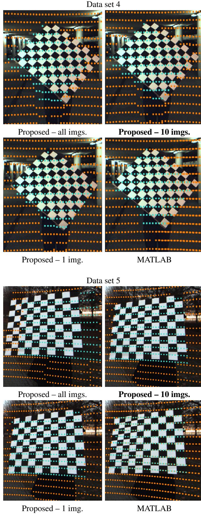
Figure 3.3: These images are from data set 4 and 5. After the calibration, the 3D points were projected back onto the image. The points corresponding to the chessboard plane can be seen in blue, all of the other back-projected LiDAR points are orange.
