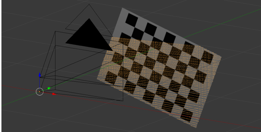
Figure 3.5: Setup of virtual LiDAR and camera in Blensor with chessboard and captured LiDAR point cloud.
