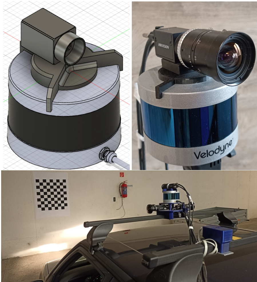
Figure 1.2: Camera-LiDAR setup. A special, 3D printed fixation used to connect the devices. Top left: 3D model of equipment. Top right: Realized Camera-LiDAR pair. Bottom: Proposed equipment mounted on the top of a car. A single chessboard is used for calibration.
