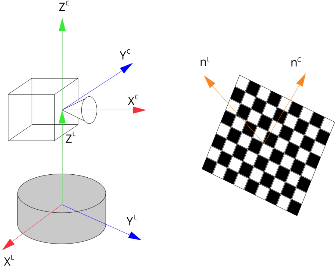
Figure 2.1: Schematic figure of Camera-LiDAR setup. Coordinate systems are highlighted by red, green and blue colors. The main goal is to estimate the rotation around axis Z_C .
