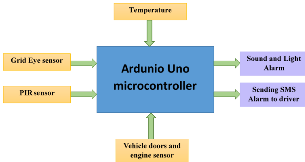
Figure 9:Block diagram of the hardware design
