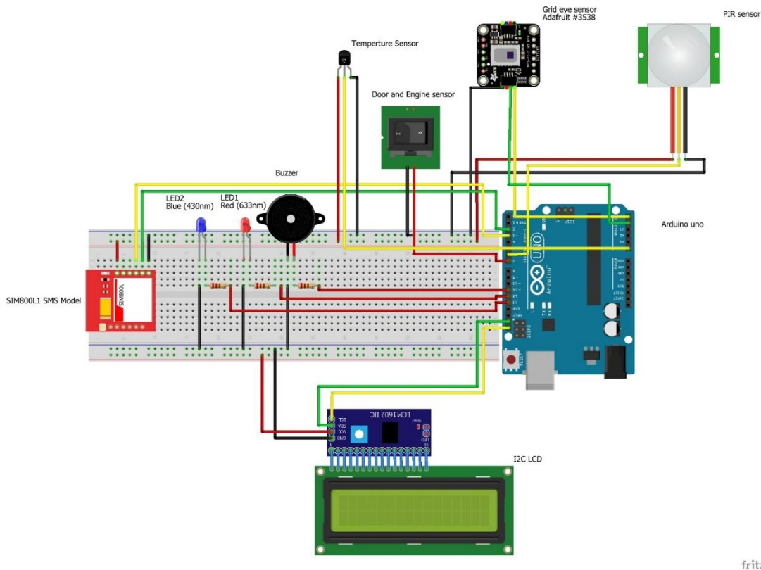
Figure 10: Circuit diagram of the hardware design
