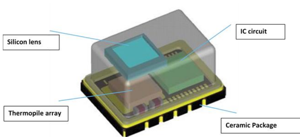
Figure 2:Grid eye package[12]
