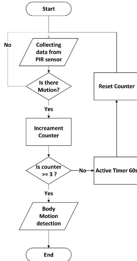
Figure 13:Flow chart of PIR sensor algorithm
