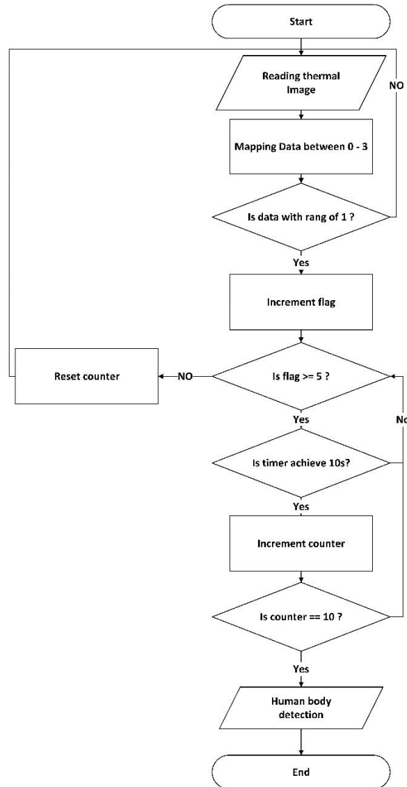
Figure 12:Flow chart of Grid Eye sensor algorithm
