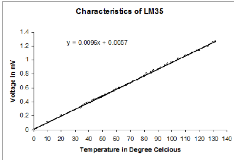
Figure 15: Characteristics of LM35 Temperature [23]
