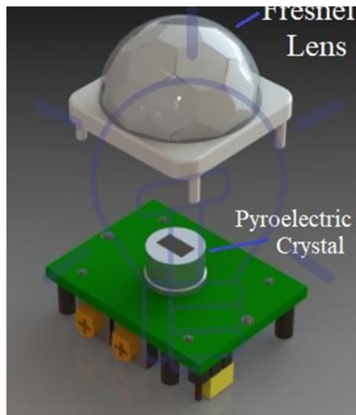
Figure 5:PIR construction [17]
