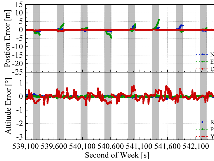
Figure 2.6: GNSS/IMU/ODO/LiDAR-SLAM navigation errors
