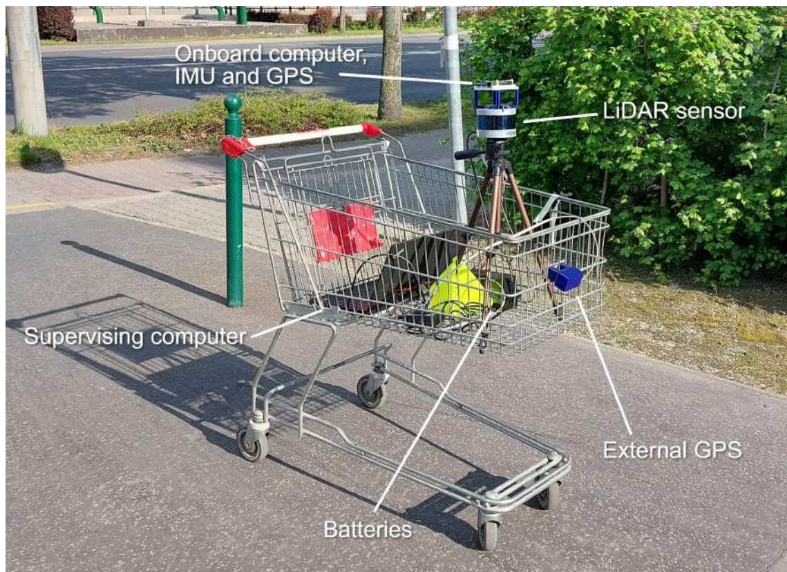
Figure 3.2: Outdoor hardware composition
