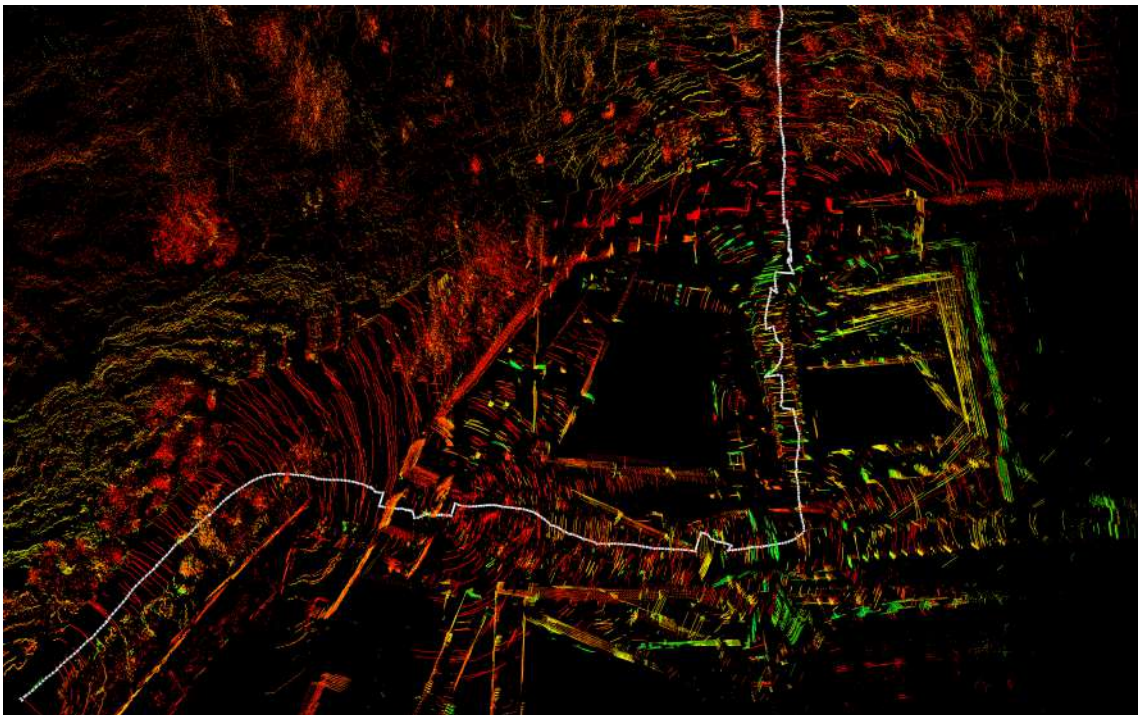
Figure 5.17: Calculated path (white) by ICP algorithm with IMU assistance
