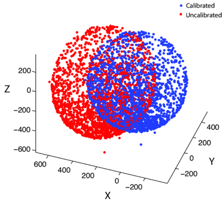
Figure 3.11: An example for magnetometer measurements before and after calibration. Axes represent magnetic field intensity in milligauss. [31]
