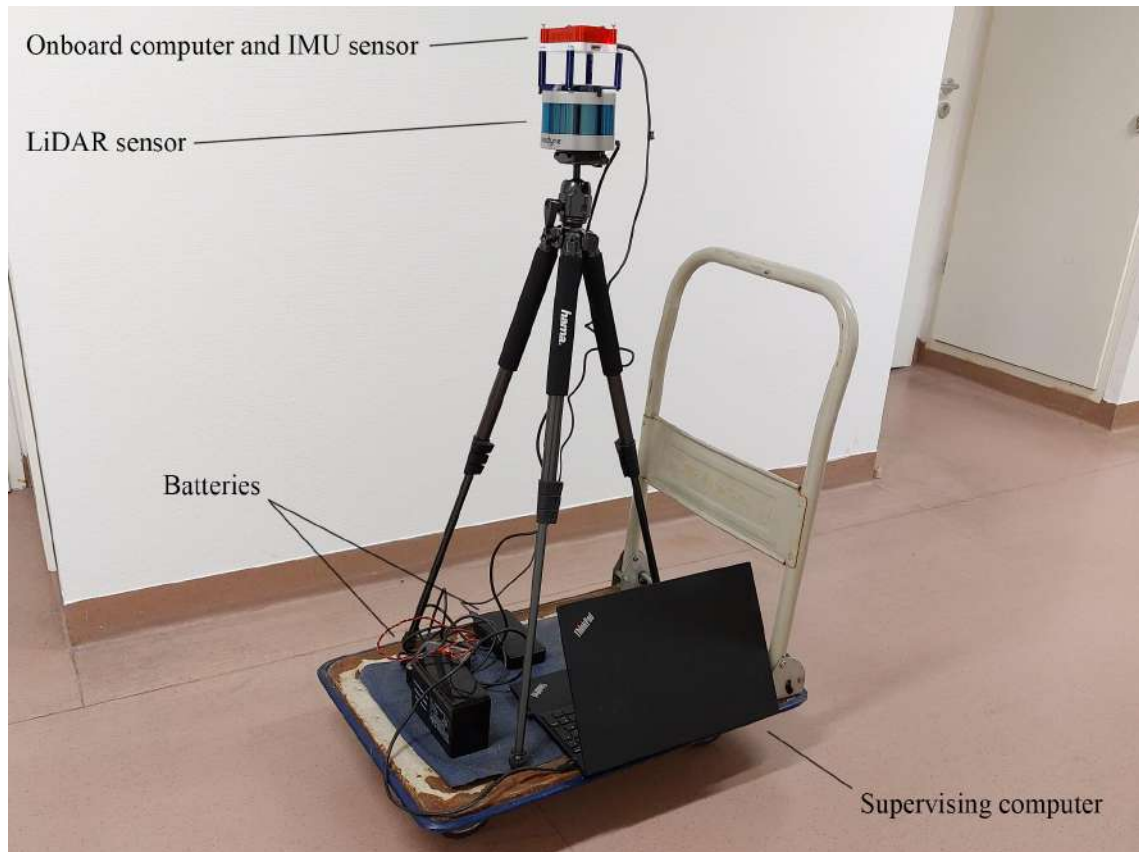
Figure 3.1: Indoor hardware composition
