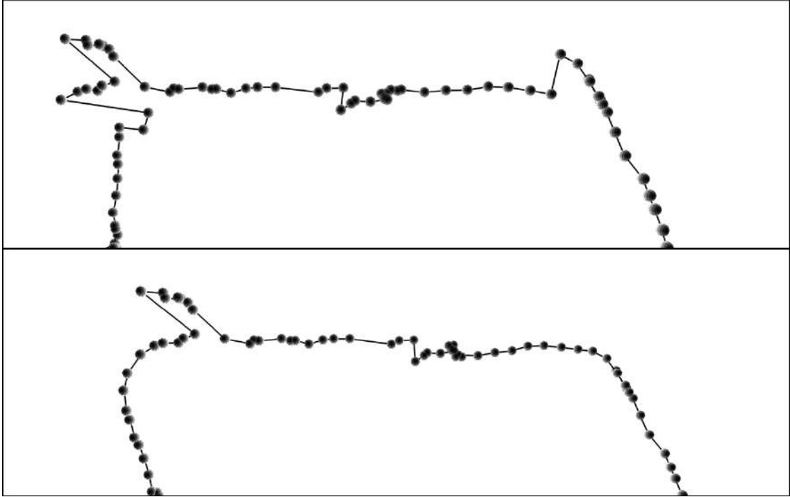
Figure 5.14: Comparison of the paths calculated via ICP (top) and IMU-assisted ICP (bottom)
