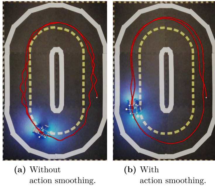
Figure 6.10: Effect of action smoothing with cubic function on robot trajectory.
