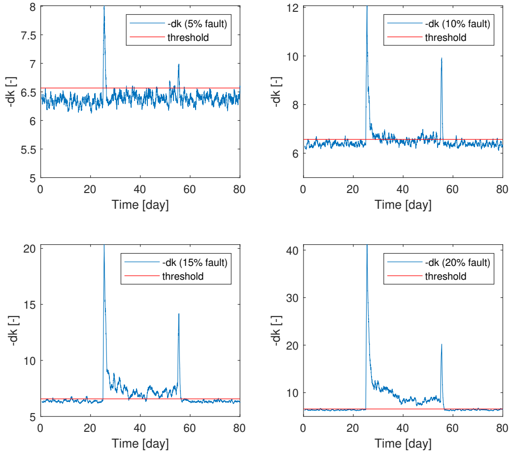
Figure 3.9: Operation with a fault: results according to different fault amplitudes. One of the setpoint changes occurs within the fault duration and one once it has been resolved, as is seen in Figure 3.8. The threshold is h = 6.57 , calculated by the 98% confidence interval of the fault-free operation. Sliding window is M = 50 . T = 8000 .
