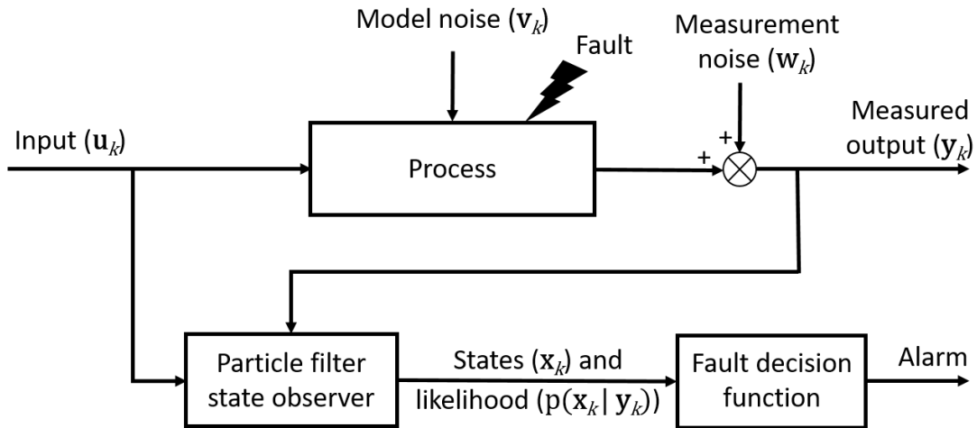
Figure 2.1: Particle filter state observer-based fault detection scheme of a process. The particle filter state observer computes the unmeasured states in light of the measured sensor data and the inputs of the process. According to the fault decision function, the faults can be detected and alarms generated. Faults can be technological faults, parameter uncertainties or sensor faults.
