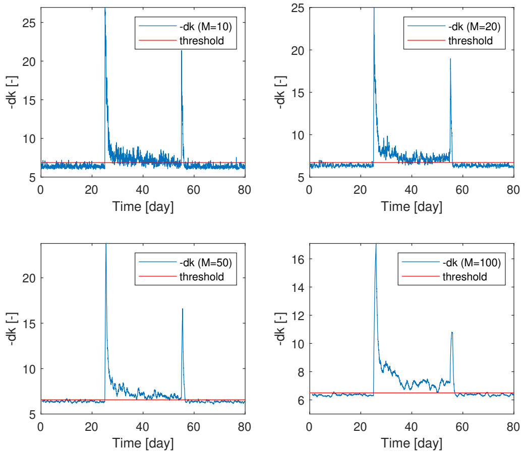
Figure 3.12: Sensitivity analysis by the sliding window ( M ): bias faults. Bias sensor faults are defined in the same way as above. M = 10, 20, 50 and 100 time steps. The 15% fault was used, that is 990 \text{ mg MLSS/L} . T = 8000 .
