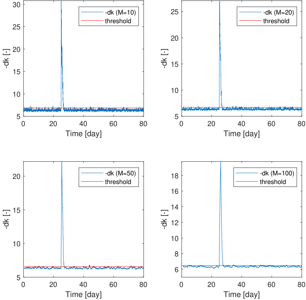
Figure 3.13: Sensitivity analysis by the sliding window ( M ): impact faults. The fault occurs from the 25th to the 26th day. M = 10, 20, 50 and 100 time steps. The 15% fault was used, that is 990 mg MLSS/L. T = 8000 .
