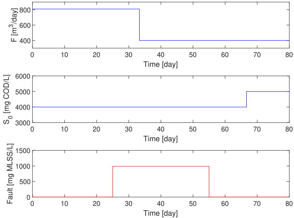
Figure 3.8: Operation with a fault: setpoint changes and the fault. The fault refers to the case of a 15% fault which is 990 mg MLSS/L. T = 8000 .
