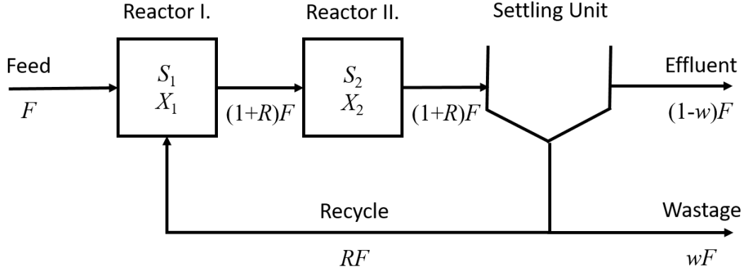
Figure 3.1: Block diagram of the standard reactor cascade (SRC) of the wastewater treatment process. The figure contains the names of the flows above the arrows and the flowrates below the arrows. F refers to the flowrate, R denotes the recycle ratio, S_i and X_i represent the concentrations of the substrate and microorganisms ( i stands for the number of the reactors), and w is the waste fraction.
