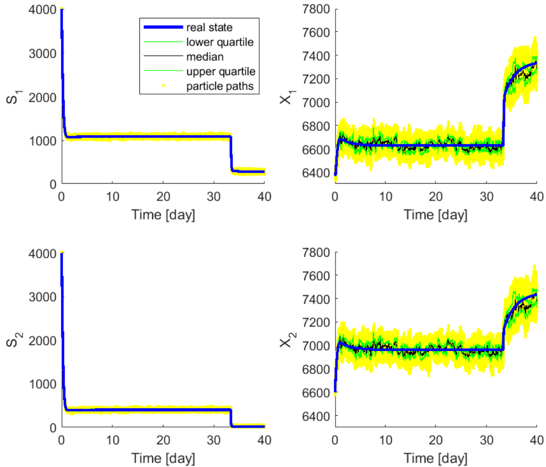
Figure 3.3: Comparison of the estimated and real states. The concentrations of the substrate are shown in mg COD/L and of the microorganisms in mg MLSS/L. Deviations of \sigma_v = 10 and \sigma_w = 25 were used for noises.
