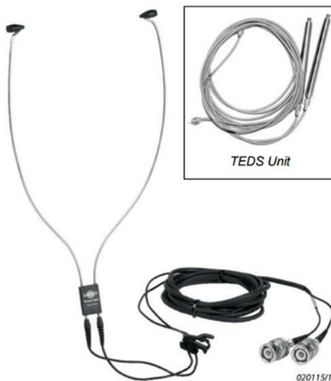
14. ábra Brüel Kjaer Binaural Microphone – Type 4101 [ https://www.bksv.com/media/doc/bp1992.pdf ]
