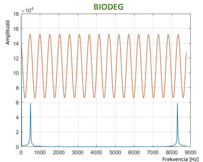
2. 500Hz 4Vpp, 2.5 V_off, SIN
