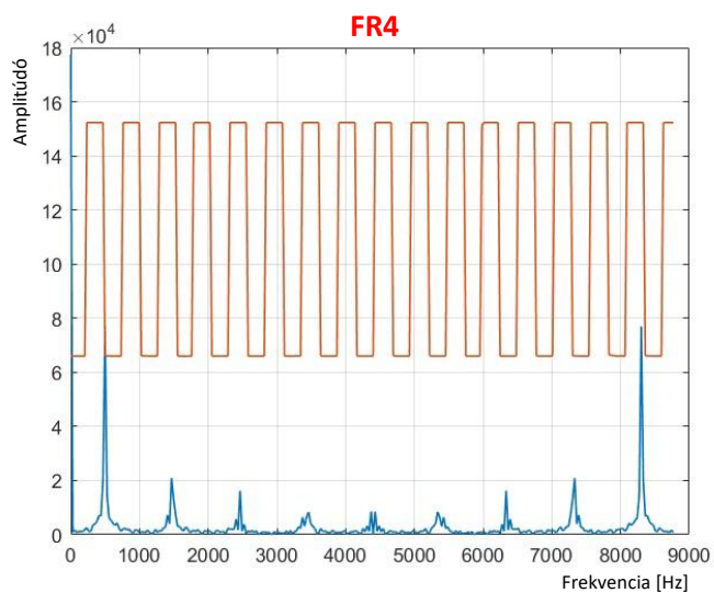
9. 500Hz 4Vpp, 2.5 V_off, SQUARE
