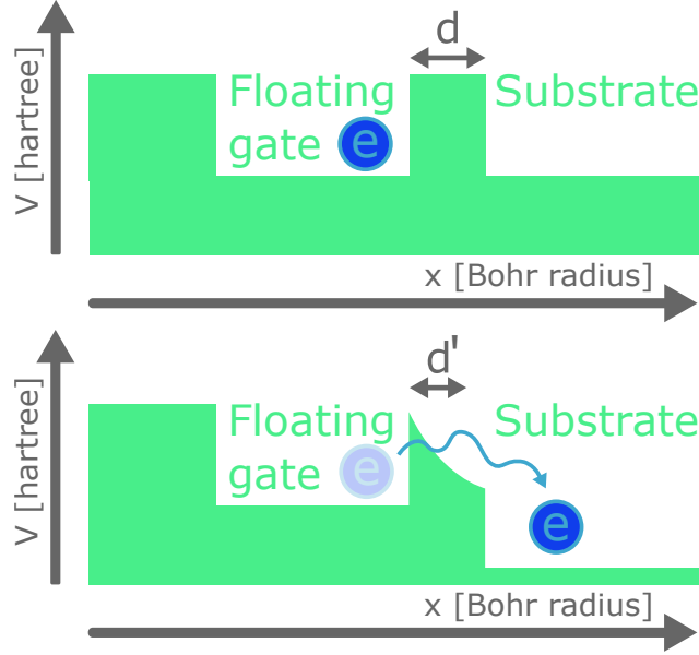
Figure 16: Fowler-Nordheim tunneling: on the upper image there is no Coulomb potential; on the image below Coulomb potential changes the shape of potential barrier causing tunneling
