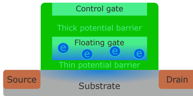
Figure 15: Schematic structure of a flash memory cell.
