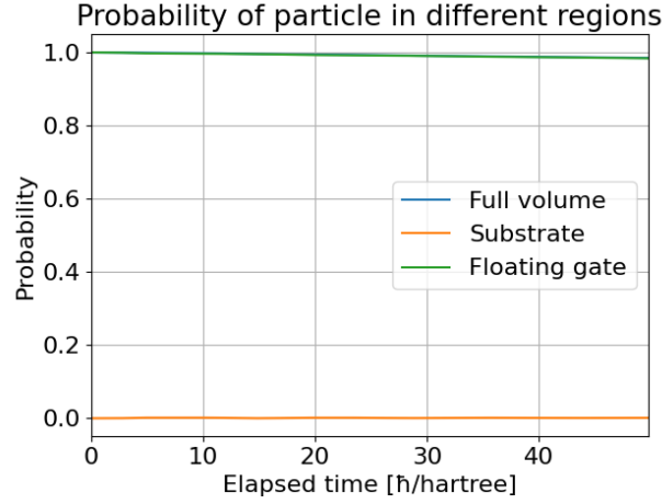
Figure 18: Storing the electron on the floating gate: there is no Fowler-Nordheim tunneling.
