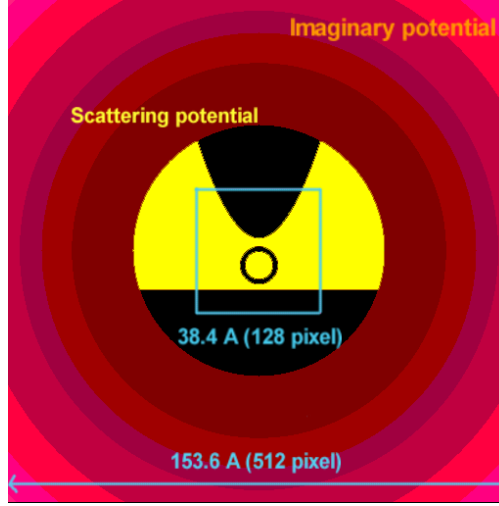
Figure 2: Calculation scheme used for the simulation of a Scanning Tunneling Microscope (STM) investigation of a carbon nanotube, as depicted by Géza István Márk. The upper black ellipse is the STM tip, the middle black ring is the cross-section of the nanotube, and the lower black region is the support electrode. The red concentric circles show the imaginary potential with increasing magnitude.
