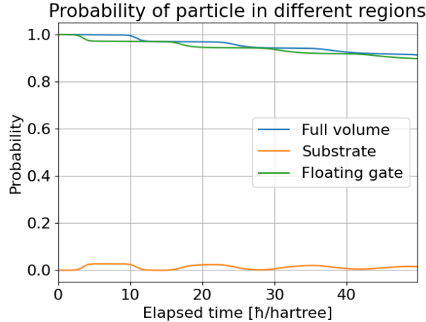
Figure 17: Flushing of the floating gate: the probability of the particle being found on the floating gate is gradually decreasing.
