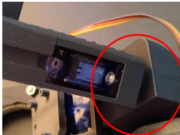
Figure A4.: An SG90 servo screwed inside the second arm part with the help of two servo screws, on the tip of that came the third arm part [highlighted]
