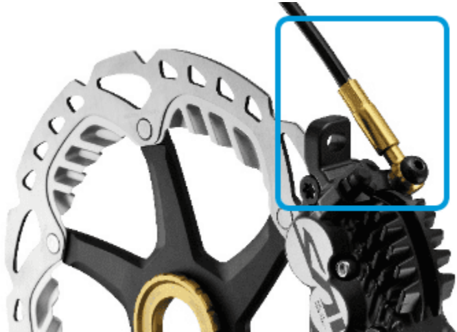
6. Ábra: Shimano Ice Technology Hose connection
