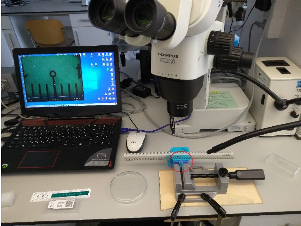
Figure 1: The measurement environment of the wobbling test.
