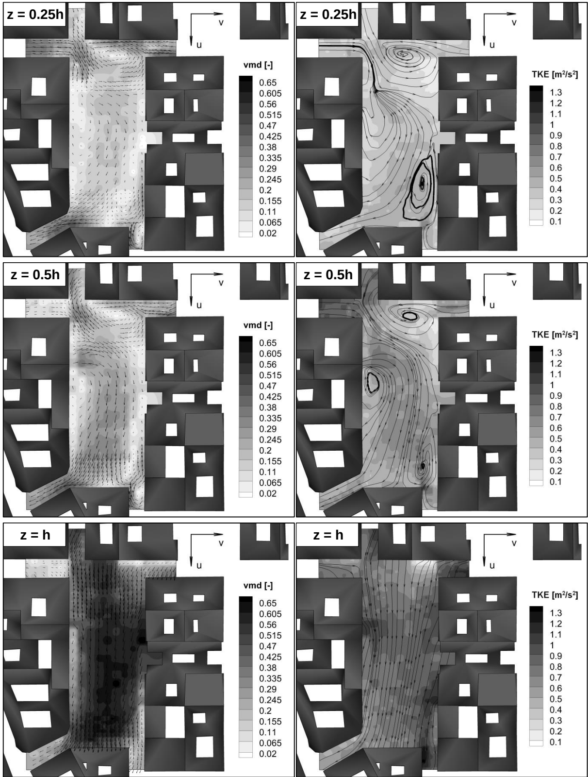
Fig. 5 Velocity and turbulent kinetic energy distributions on horizontal planes (vmd: dimensionless horizontal mean velocity magnitude)
