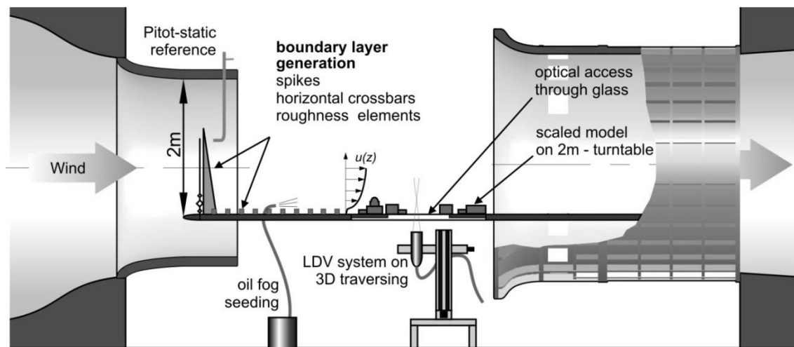
Fig. 1 The wind tunnel test section
