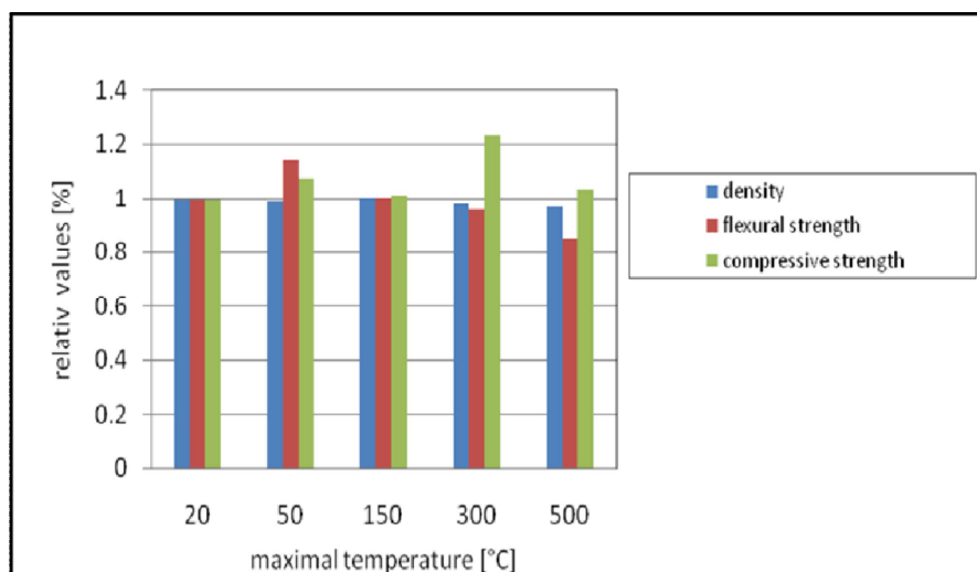
Figure 5. Density (based on CT measurements) as well as flexural and compressive strength measurements (based on mechanical test)
