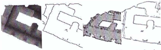
Figure 3: Outer edge detection's assembly - projection (z-image) - edge detection - elevation into the 3D space - segment fitting.
