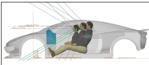
Figure 8: The Ergonomics Simulations: The Vision (Field of View) Evaluation
