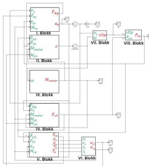
Figure 5 The block diagram of the simulation program
