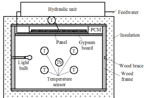
Figure 11 Section drawing of the adiabatic box
