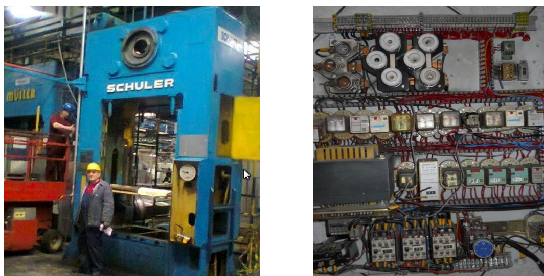
Figure 2 Press frame closed undergoing modernization; Analog electric panel.
