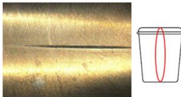
Figure 11 Pulling traces
