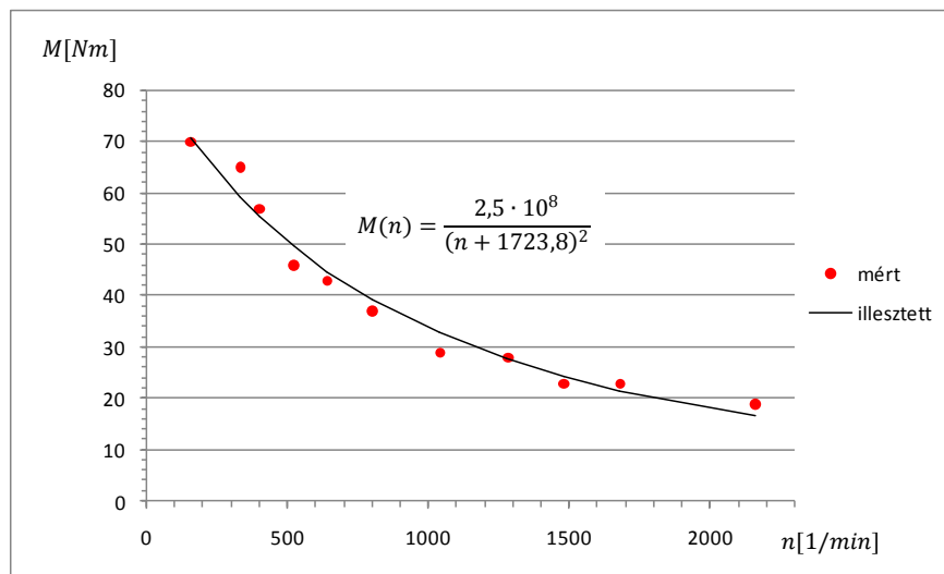
Figure 8 Torque-speed curve of DC motor
