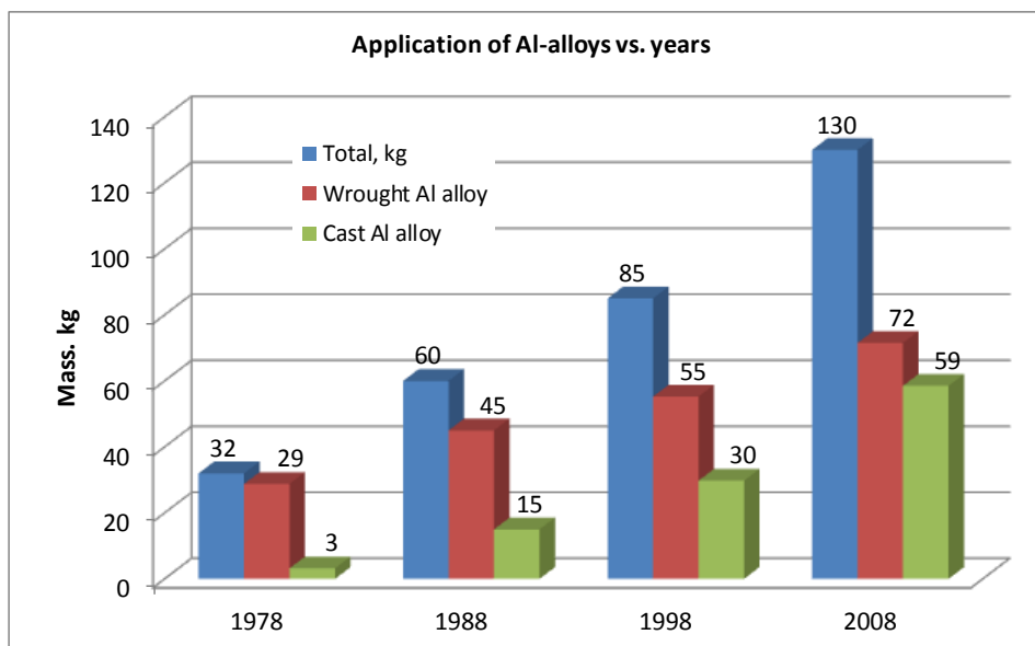
Figure 3 Application trends of aluminum wrought and cast alloys in car manufacturing [6]
