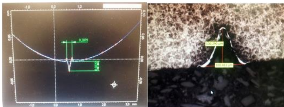
Figure 21 Inner crack dimension measurement with Mahr Perthometer (left) and optical microscope (right)
