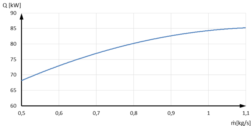
Figure 3 Extractable heat power as a function of the mass flow (CO 2 ) ( t_{\text{cond}}=12\text{ }^{\circ}\text{C} )
