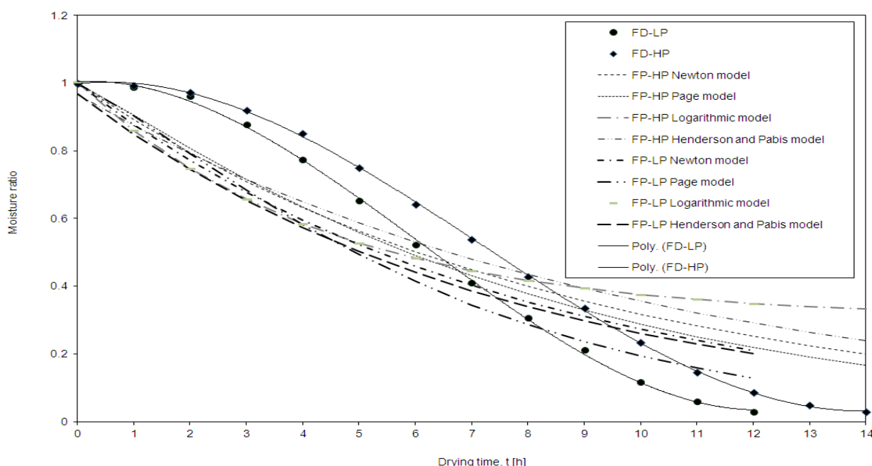
Figure 2 Variations of moisture ratio as a function of drying time for FD of lemon balm
