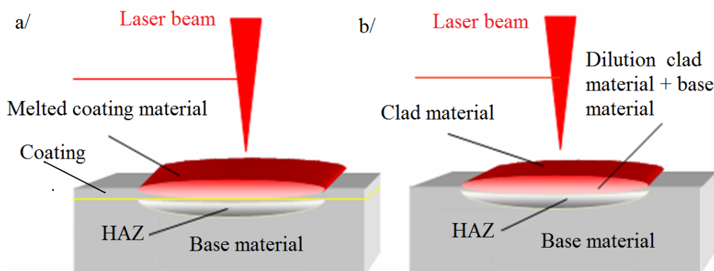
Figure 1 Laser surface treatment techniques; (a) laser surface remelting, (b) laser cladding
