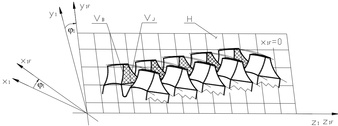
Figure 2 Defining H face surface and V_{J,B} cutting edges in case of planar face surface
