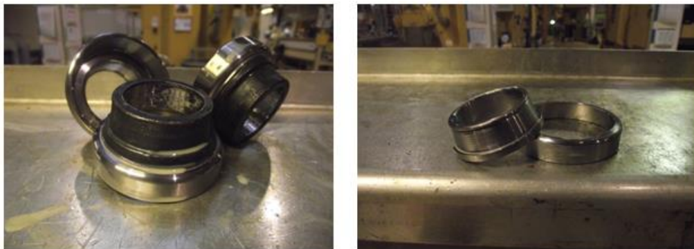
Figure 2 Lateral grinded tower ring (left) and separated rings (right)
