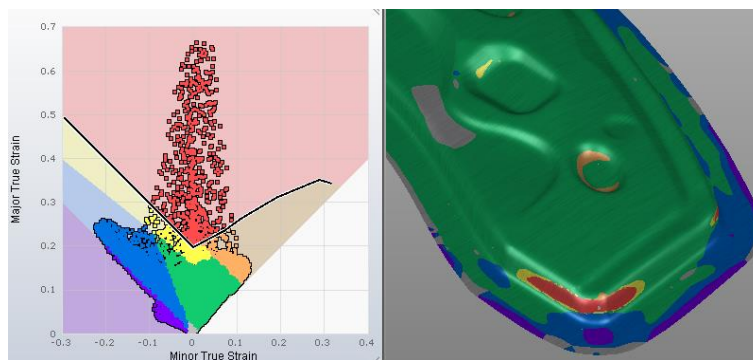
Figure 2.: Numerical simulation with EN AW 5754 material
