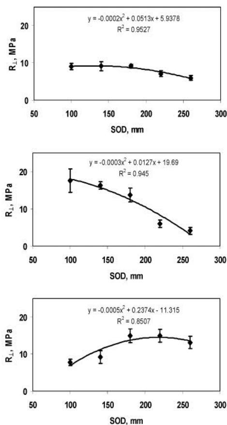
Figure 6. Normal component of coating bond strength, R_{\perp} From top to bottom: DuroTec, HardTec, LubroTec
