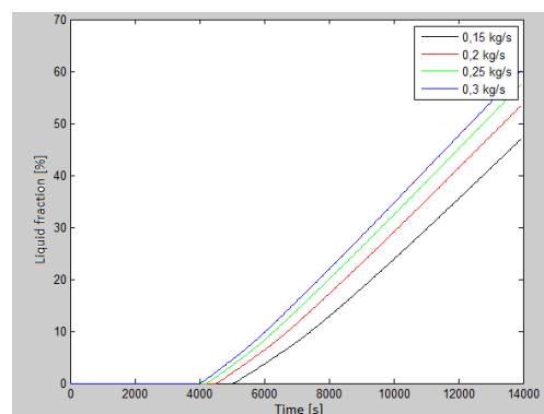
Figure 8 Liquid fraction in the function of water mass flow
