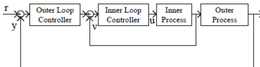
Figure 2 General block diagram of cascade control (Geng, 2014)
