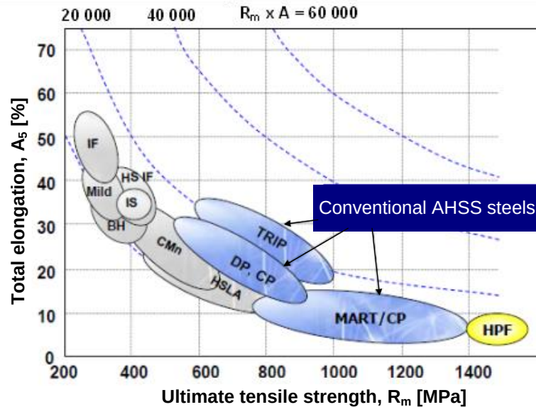
Figure 1 Tensile strength vs. total elongation for various steel grades [3]
