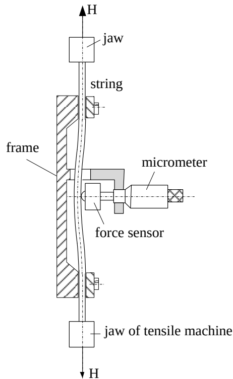
Figure 2. Measuring setup
