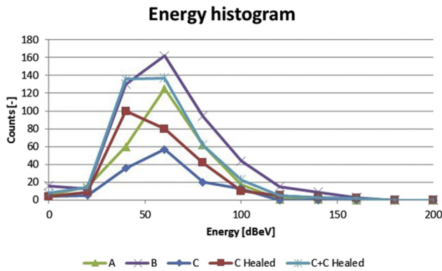
Fig. 5. AE energy histograms of the tested samples.
