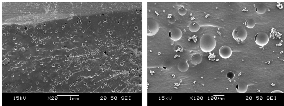
Fig. 8. SEM micrographs of sample "C Healed".
