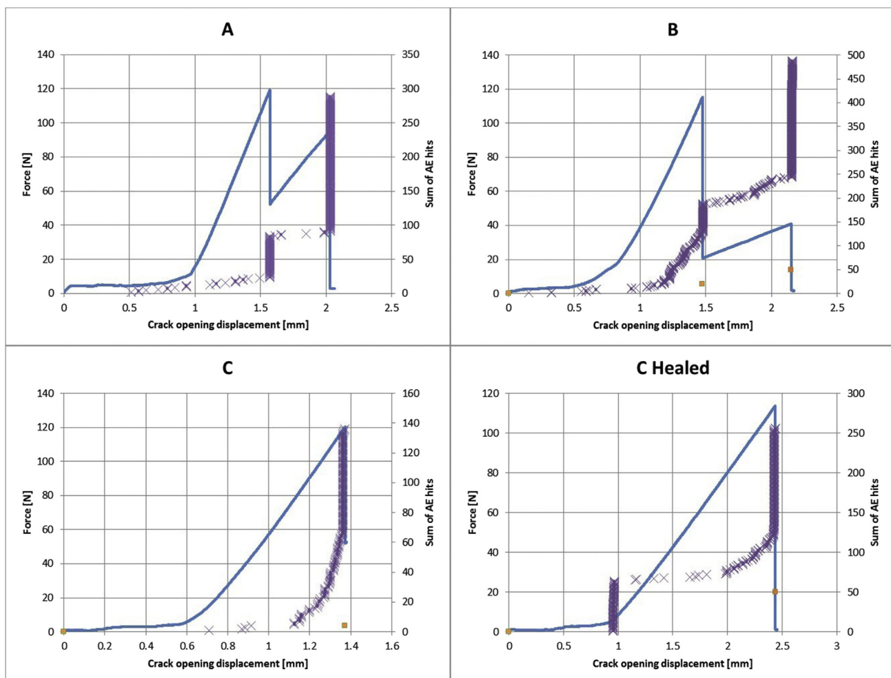
Fig. 3. Recorded force and sum of AE hits curves of an unfilled (A), epoxy microcapsule filled (B), and a self-healing specimen before (C) and after healing (C Healed) as a function of crack opening displacement.
