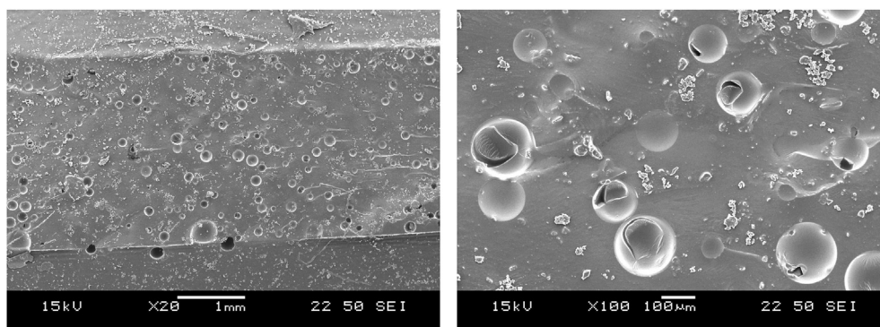
Fig. 7. SEM micrographs of sample "B".
