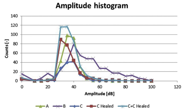
Fig. 4. AE Amplitude histograms of the tested samples.
