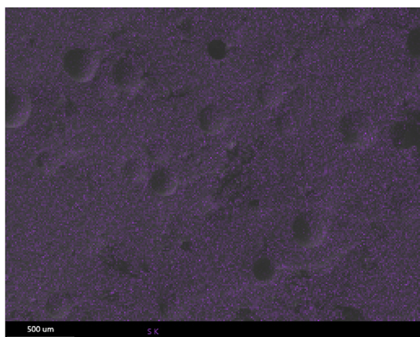
Fig. 9. SEM micrograph of sample "C Healed" with the detected sulfur location EDS overlay (purple dots). (For interpretation of the references to colour in this figure legend, the reader is referred to the web version of this article.)
