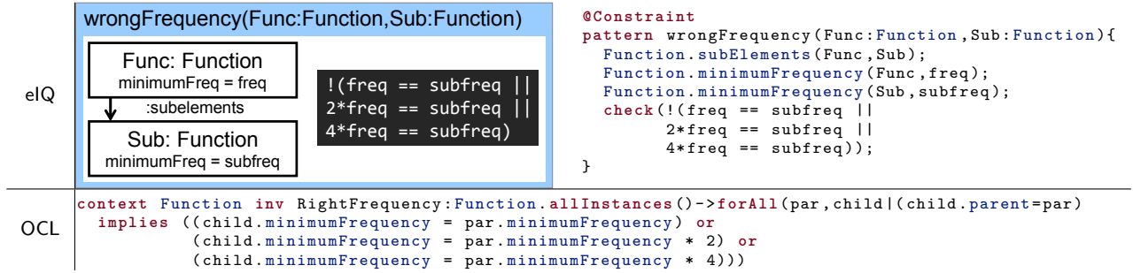
Fig. 7: Constraint for the frequency of the subfunctions
