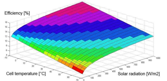
Fig. 2. Efficiency of the examined solar module
