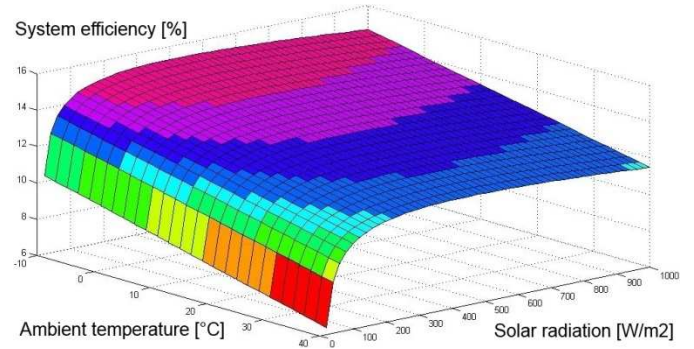
Fig. 4. Efficiency of a PV system
