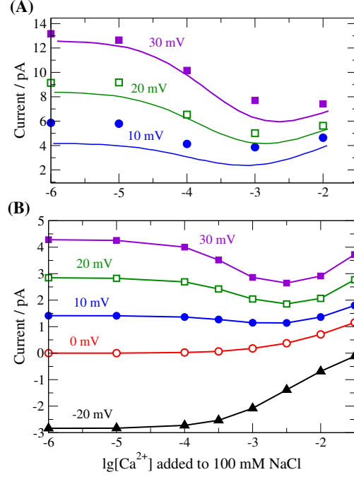
Figure 5: The added \text{CaCl}_2 experiment considered by Gillespie et al. [30]. \text{CaCl}_2 is added to a constant background of 100 mM NaCl to the left hand side of the membrane at different voltages (ground is on the right). \text{Ca}^{2+} concentration is micromolar on the right side. The dimensions of the access and bulk regions are 20 and 10 Å, respectively. The resolution of the grid is 2 \times 2 Å. Panel (A) replots the results of Fig. 1B of Ref. [30]. Symbols are experiments, while lines are results of NP+DFT calculations. Panel (B) shows the results of our NP+LEMC calculations.
