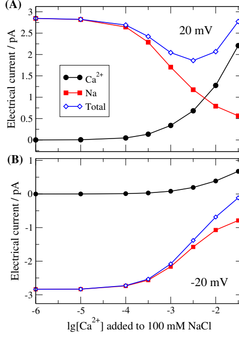
Figure 6: Electrical currents for the situation depicted in Fig. 5. Currents carried by the different ions (and their sum) are plotted for voltages (A) 20 mV and (B) -20 mV.
