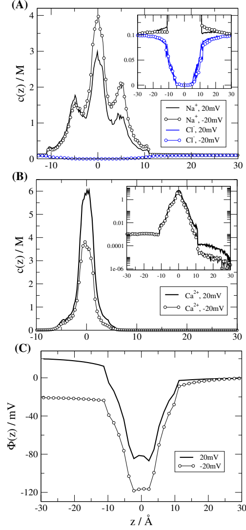
Figure 7: Profiles for the case depicted in Fig. 5 for c_{\text{L}}^{\text{Ca}^{2+}} = 1 \text{ mM} at the two indicated voltages. Panel (A) shows \text{Na}^+ and \text{Cl}^- concentration profiles (the inset magnifies the small concentration regime), panel (B) shows the \text{Ca}^{2+} concentration profiles (the inset uses logarithmic scale for the ordinate), while panel (C) shows the electrical potential profiles.
