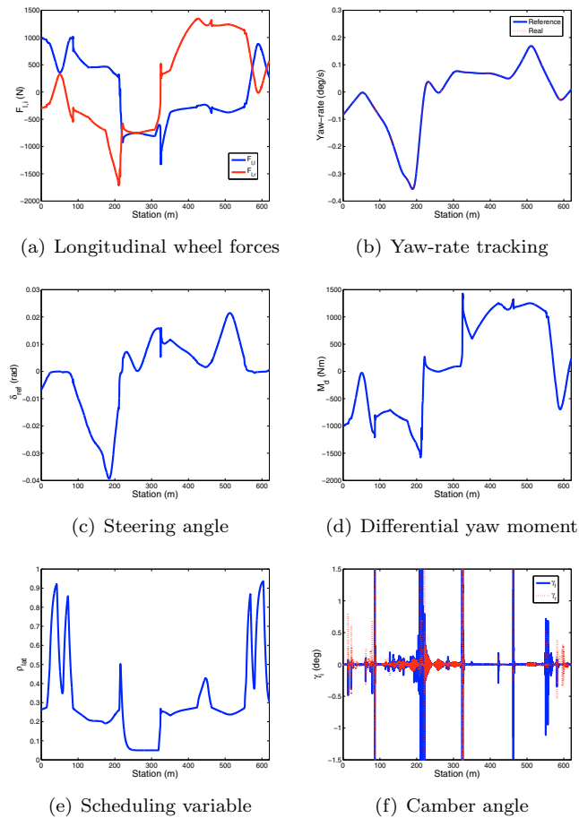
Fig. 7. Signals of the trajectory tracking
