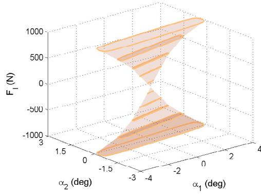
Fig. 3. Reachable sets of the variable-geometry suspension
