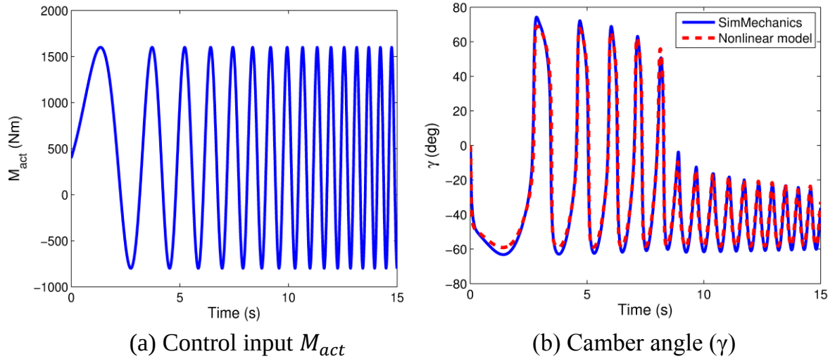
Figure 3: Model validation - Chirp signal
