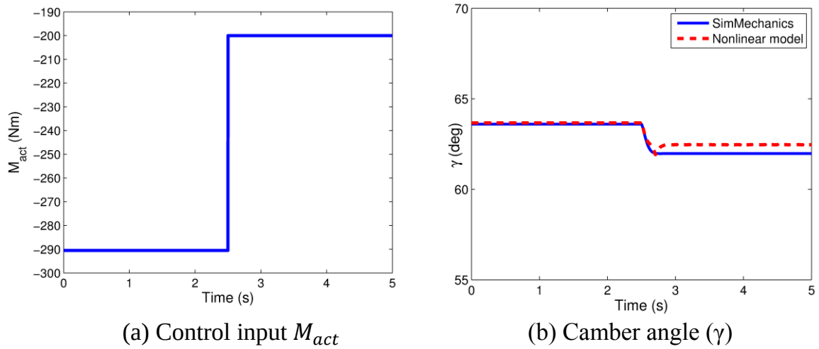
Figure 4: Model validation - Step signal
