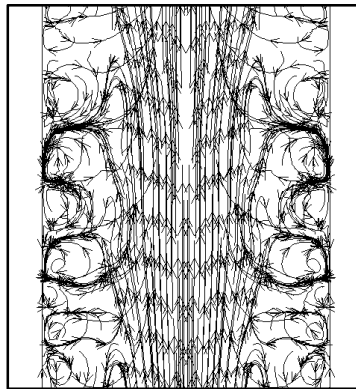
Figure 9a. Pathlines of the secondary flow D = 10 mm
