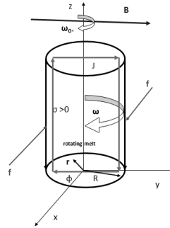
Figure 1. The force system in the inductor
