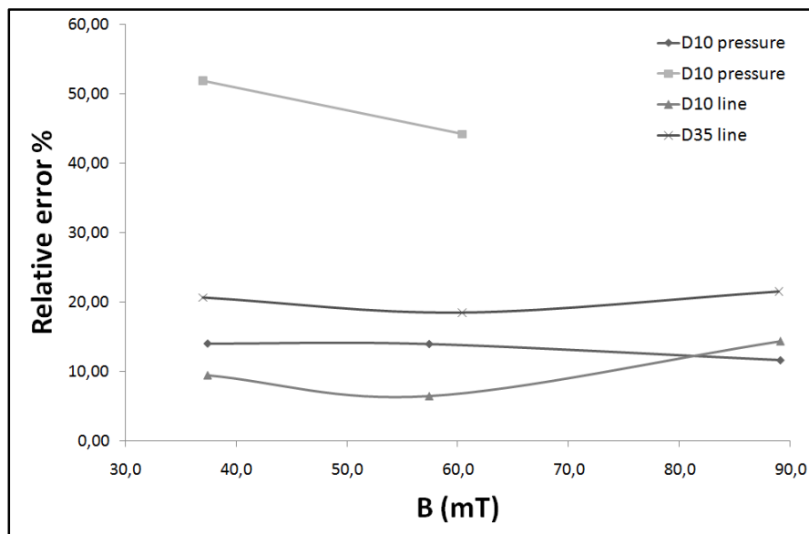
Figure 12. Relative error on the angular velocity measured with both methods as a function of the induction
