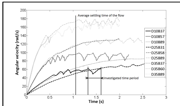
Figure 5. Angular velocities as a function of time from 0 seconds
