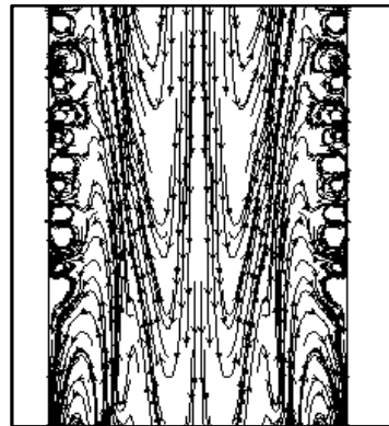
Figure 9b. Pathlines of the secondary flow D = 35 mm
