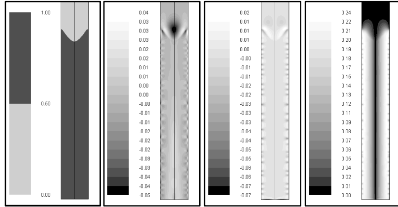
Figure 10a. Figure 10b. Figure 10c. Figure 10d. Contours of: (10a.) volume fraction of gallium, (10b.) axial velocity magnitude, (10c.) radial velocity magnitude and (10d.) tangential (swirl) velocity magnitude. Scale bar on b. c. and d. is in m/s; D = 10 mm, B = 37 mT
