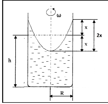
Figure 4. Sketch for computing the angular velocity
