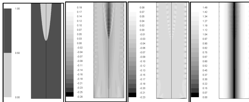
Figure 11a. Figure 11b. Figure 11c. Figure 11d. Contours of: (11a.) volume fraction of gallium, (11b.) axial velocity magnitude, (11c.) radial velocity magnitude and (11d.) tangential (swirl) velocity magnitude. Scale bar on b. c. and d. is in m/s; D = 35 mm, B = 37 mT
