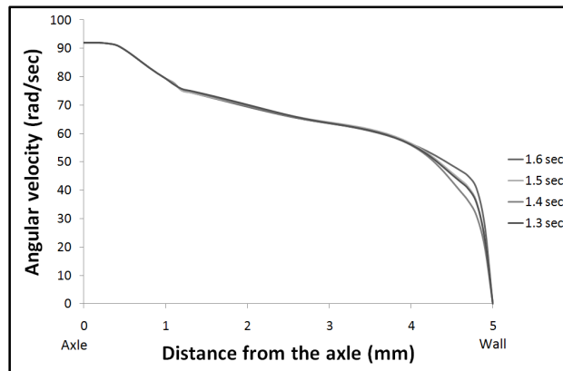
Figure 6. Angular velocity plotted from the axle to the wall, D = 10 mm, B = 37 mT
