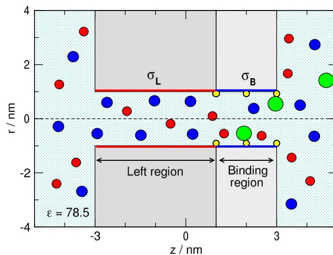
Fig. 1. Schematics of the cylindrical pore that is divided into two regions. The left region of length H_L = 4 nm carries \sigma_L surface charge that determines the main charge carrier of the pore. The right region is the “binding region”, where the binding sites are located (indicated by small yellow spheres on the wall). The length of this region is H_B = 2 nm and can carry \sigma_B surface charge. The radius of the pore R_{\text{pore}} = 1 nm in this study. The green sphere is the analyte ion, X^+ , that is bound to the binding site if it overlaps with the yellow sphere. The blue and red spheres are the cations ( K^+ ) and anions ( Cl^- ) of the electrolyte, respectively. (For interpretation of the references to color in this figure legend, the reader is referred to the web version of this article.)
