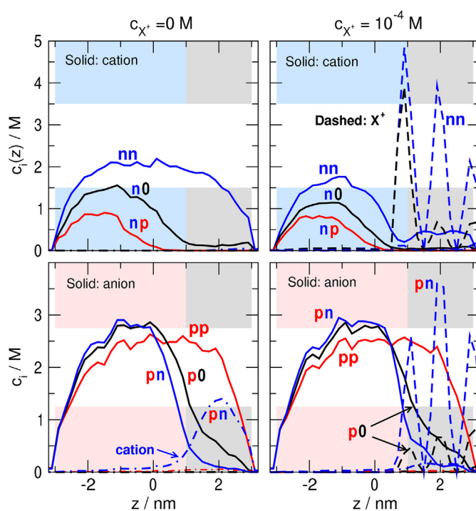
Fig. 5. Concentration profiles for c_X = 0 M (left panels) and c_X = 10^{-4} M (right panels) for the ON states. Profiles for X^+ are shown with dashed lines. Solid lines show the profiles for the main charge carriers, while the dot-dashed lines show the profiles for the other ion. Top panels show the results for the nn , n0 , and np geometries with solid lines being the cation profiles. Bottom panels show the results for the pp , p0 , and pn geometries with solid lines being the anion profiles. The colors are determined by the \sigma_B charge (blue for n , black for 0 , and red for p ). (For interpretation of the references to color in this figure legend, the reader is referred to the web version of this article.)
