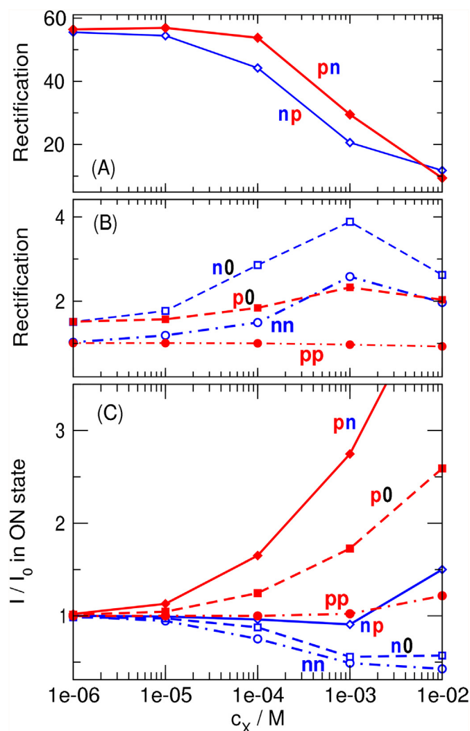
Fig. 4. The dependence of the device functions on c_X for the various charge patterns. Panels A and B show the rectification defined as I_{ON}/I_{OFF} (for the n0 and np charge patterns -200 mV is the ON state, while for the p0 and pn charge patterns 200 mV is the ON state). Panel A shows the large rectifications characteristic of the bipolar pores ( np and pn ). Panel B shows the rectification for the other geometries. Panel C shows the ON-state I/I_0 ratio with I_0 being the current at c_X = 0 M.
