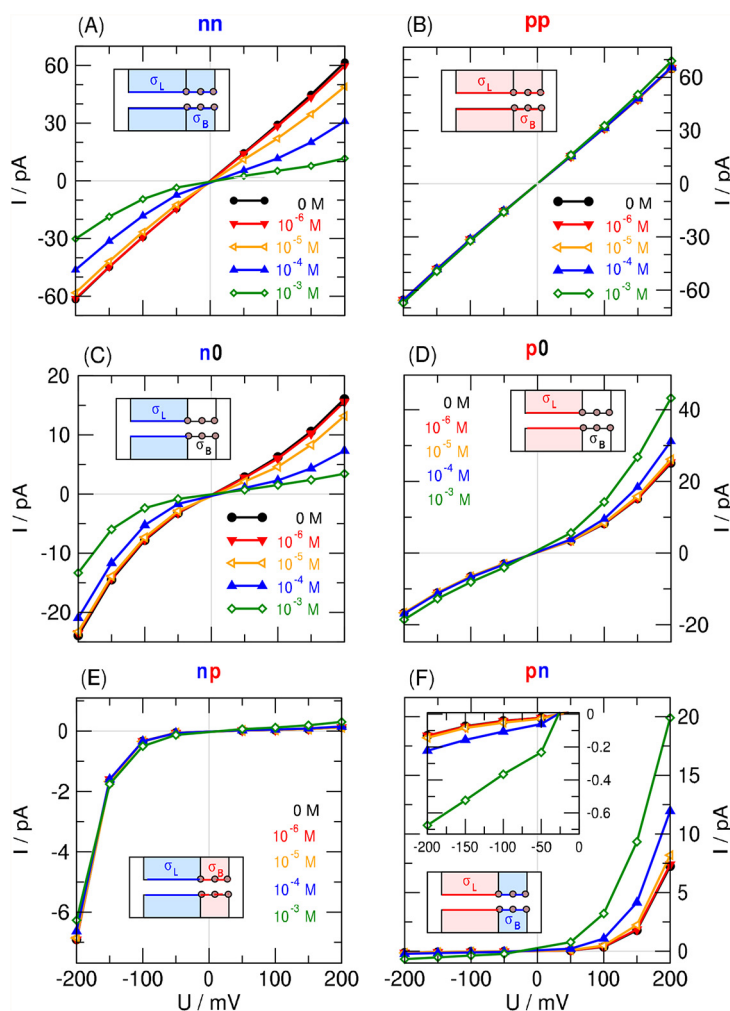
Fig. 2. Current-voltage curves ( I vs. U ) for the different charge patterns. Left panels (A, C, and E) refer to charge patterns, where the left region is negative, \sigma_L = -1 e/m 2 , while right panels (B, D, and F) refer to charge pattern, where the left region is positive, \sigma_L = 1 e/m 2 . Top panels (A and B) refer to uniformly charged pores, nn and pp . Middle panels (C and D) refer to unipolar pores, n0 and p0 . Bottom panels (E and F) refer to bipolar pores, np and pn . For explanation of notations, see the main text. The values of \sigma_B and \sigma_L take the values -1 , 0 , or 1 e/nm 2 . Every panel shows results for different X^+ concentrations from 0 to 10^{-3} M. The inset in panel F shows the OFF currents for the pn geometry.
