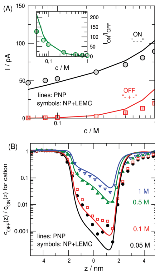
Fig. 6 (A) Concentration dependence of the current in the ON (“– – –”) and OFF (“– + –”) states. The inset shows the I_{\text{ON}}/I_{\text{OFF}} ratio. (B) Ratio of cation concentration profiles in the OFF and ON states for different bulk concentrations.
