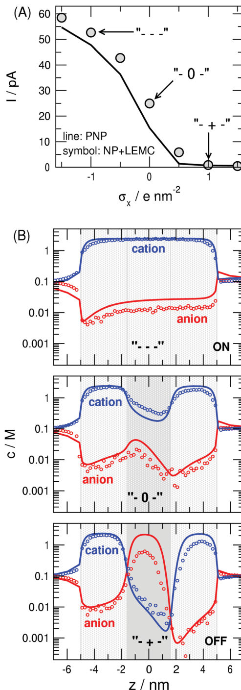
Fig. 2 (A) Current as a function of \sigma_x while \sigma_n = -1 \text{ e nm}^{-2} is kept fixed. Selected charge patterns are indicated with “– – –” (ON), “– 0 –”, and “– + –” (OFF). Increasing \sigma_x makes the x region more positive, so the I(\sigma_x) function is monotonically decreasing. (B) Concentration profiles for these selected charge patterns. Widths of the regions are H_x = 3.2 and H_n = 3.4 nm, electrolyte concentration is c = 0.1 M, voltage is 200 mV. Symbols and lines denote NP + LEMC and PNP results, respectively, here and in all the remaining figures unless otherwise stated.
