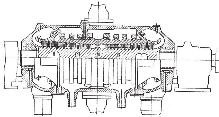
Figure 1 Longitudinal section of a high-pressure cylinder with double casing and shrink rings for the inner case
