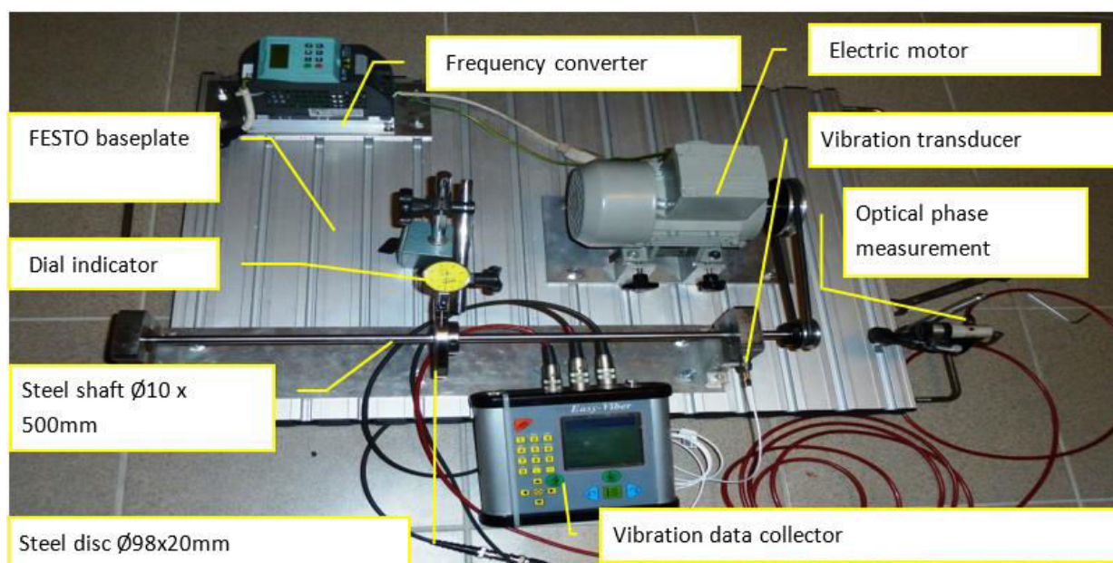
Figure 1 Test rig developed at the Óbuda University
