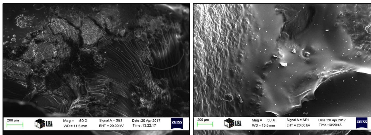
Figure 4 SEM microscopy results of Coconut oil mixed sample on 50x magnification
