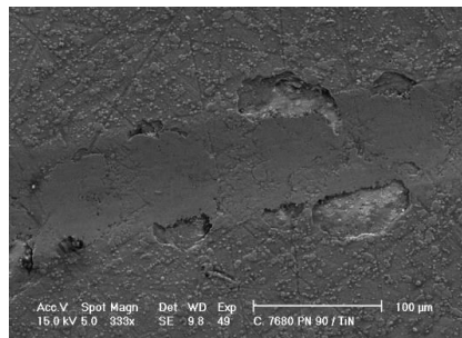
Figure 2 SEM morphology of scratch test: pn/TiN(PVD).
