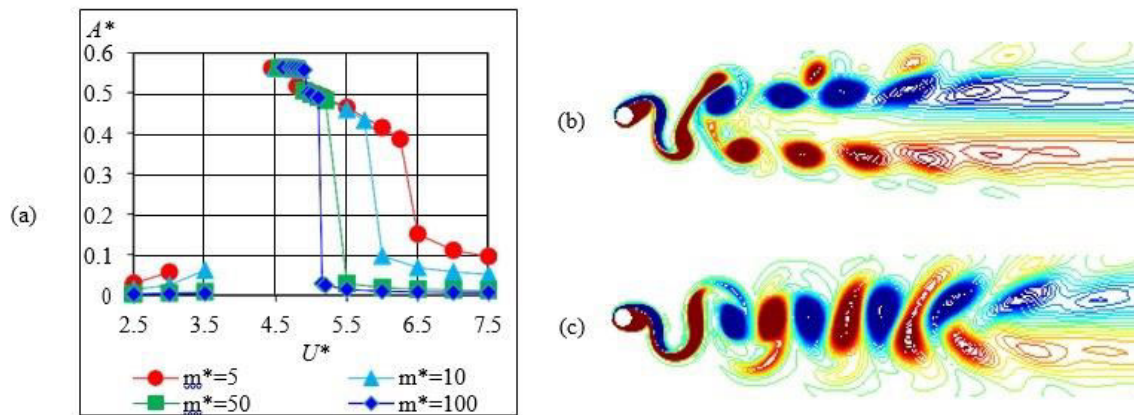
Figure 1 Dimensionless oscillation amplitude vs. reduced velocity (a) and vortex structures at U^*=4.79 (b) and U^*=4.80 (c) at t=800 for m^*=5
