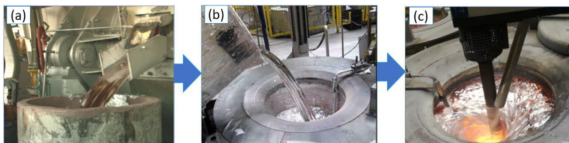
Figure 1 The stages of melt preparation: a) pouring from melting furnace, b) melt transport to holding furnace, and c) melt processing
