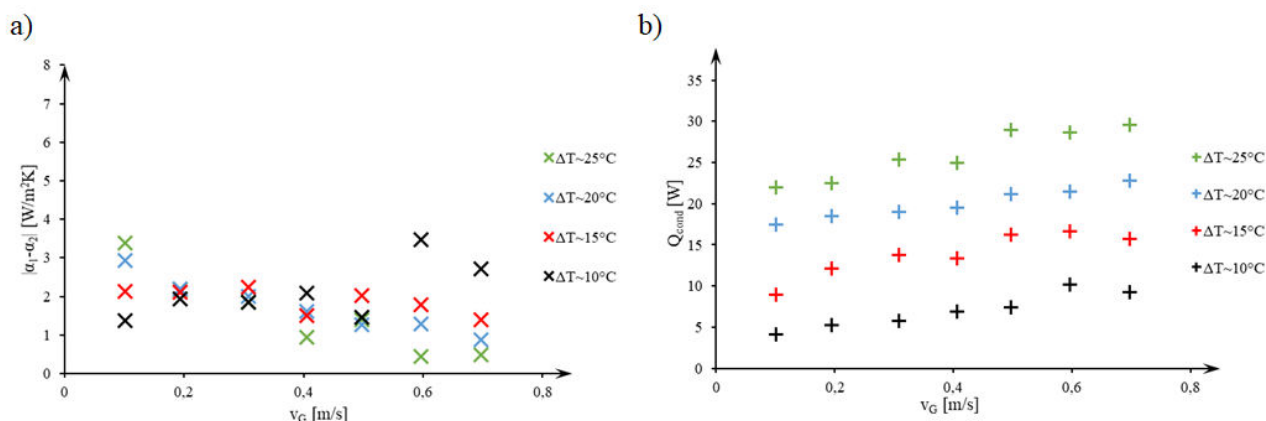
Figure 1 a) Difference between the heat transfer coefficients as a function of air velocity, b) Conductive heat as a function of air velocity
