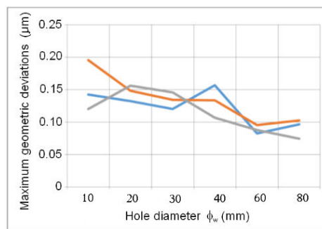
Figure 3 Size of the maximum geometric deviations of circularity of the machined surface with diameters in the range \phi_w = 10.0 - 80.0 mm after WEDM with wire electrode \phi_e = 0.25 mm.
