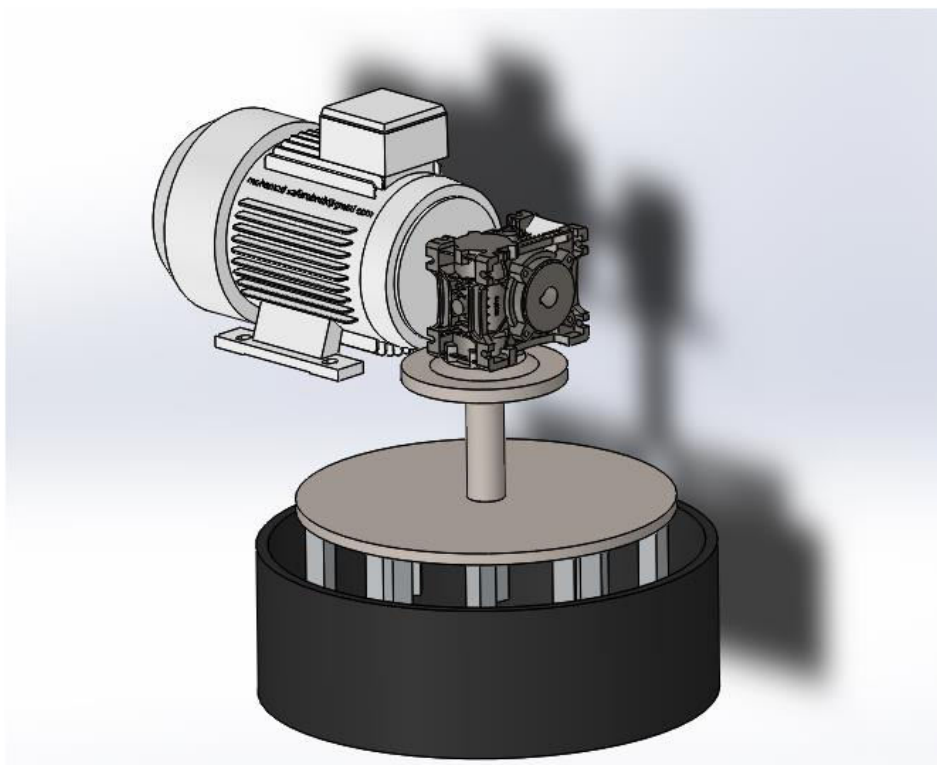
Figure 1 The slurry-pot abrasive wear test device
