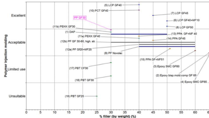
Figure 2 Influence of quantity of filler on the injection mouldability of the alternative materials of the impeller
