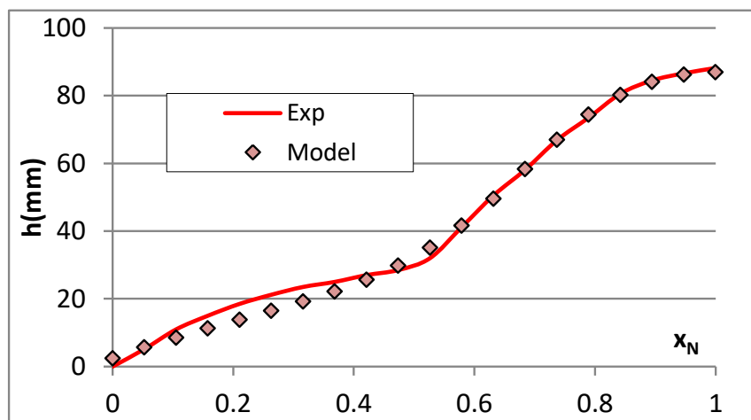
Figure 3 Example of model prediction of effective road profile, compared to experiment result
