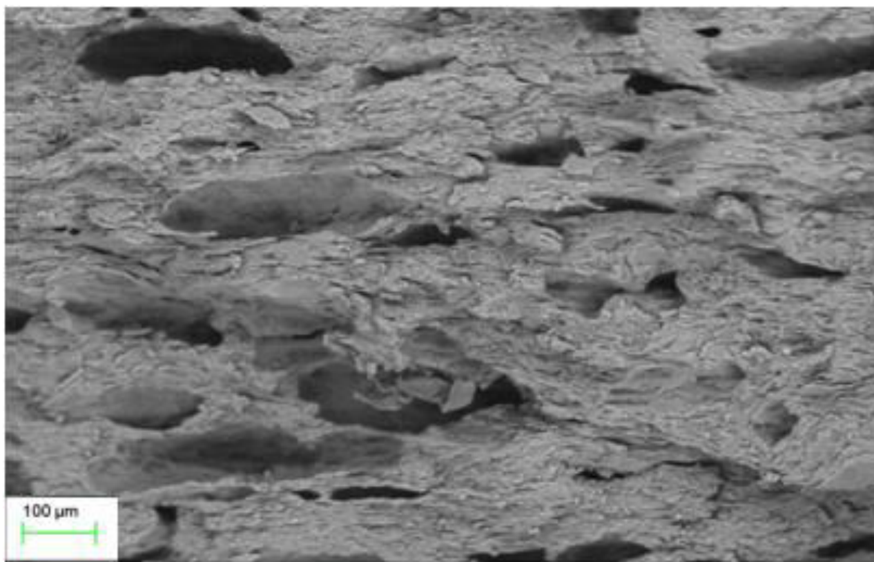
Figure 1 Scanning Electron Microscope fractured structure of PVC/LDPE foam
