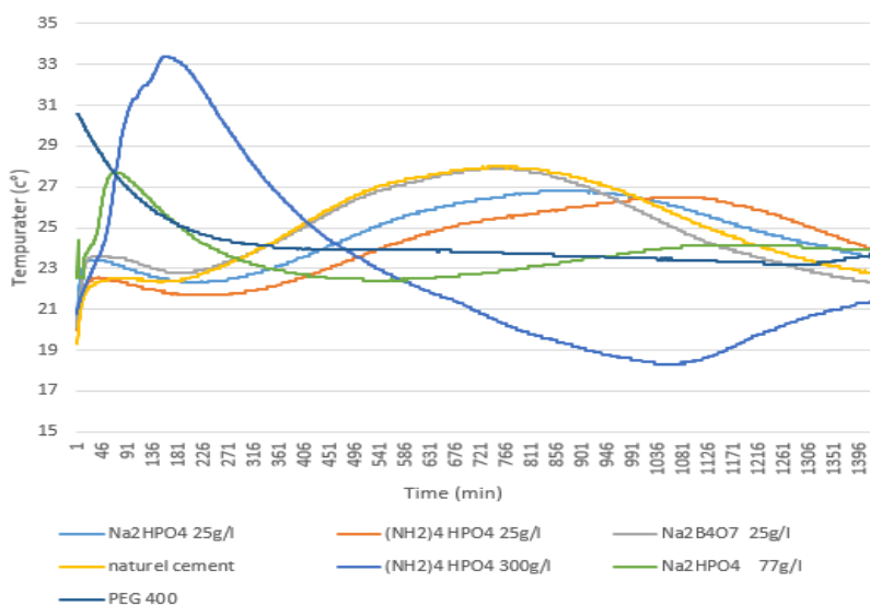
Figure 2 Hydration test.
