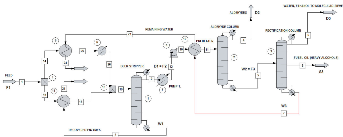
Figure 1 Model of the heat-integrated bioethanol distillation plant (CaseHI-A)
