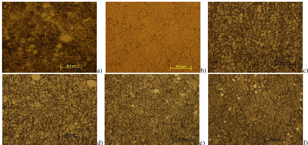
Figure 2 Representative microstructures of samples in (a) delivery condition, (b) quenched and tempered at 200°C, (c) quenched and tempered at 510°C (d) quenched and triple tempered ( 510°C+480°C+480°C), (e) quenched, cryrogenically treated and tempered at 510°C (e) quenched, cryrogenically treated and triple tempered (510°C+480°C+480°C) after etching with nital 2%. N_{original}=1000x
