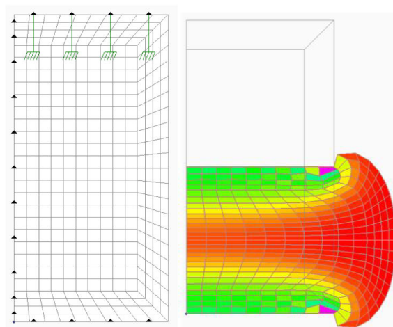
Figure 4 Deformation state of a rubber bumper with the use of quadrilateral elements and mesh design
