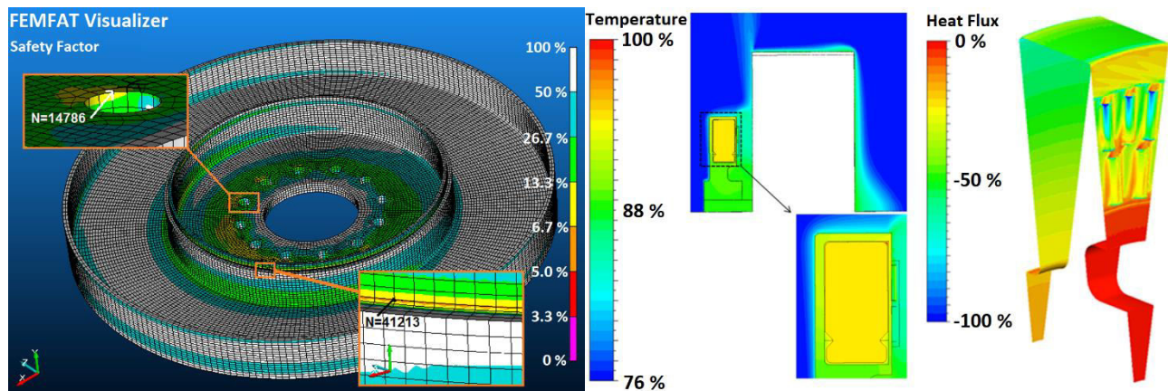
Figure 2 FEMFAT fatigue analysis result with critical points (left side) and heat transfer result (right side)
