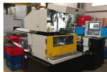
Figure 1 FANUC ALFA C600iA electro-erosion machine
