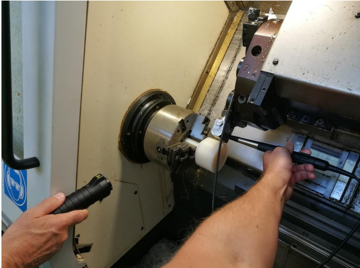
Figure 2 The setup for measuring the spindle speed, the vibration in tangential direction, and the shock pulse in axial direction
