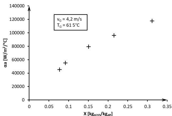
Figure 2 Volumetric heat transfer coefficient versus moisture content dry basis
