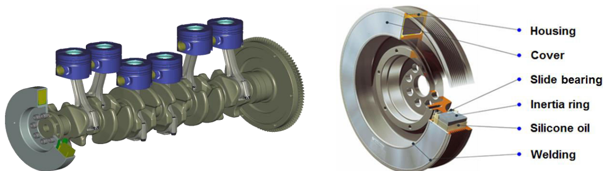
Figure 1 Torsional vibration damper mounted onto the crankshaft (left) and the structure of a visco-damper (right)
