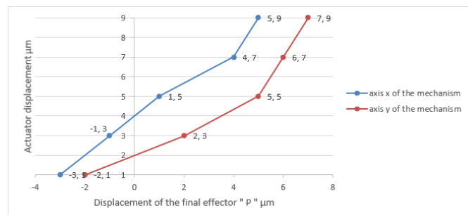
Figure 5c Rectangular joint profile
