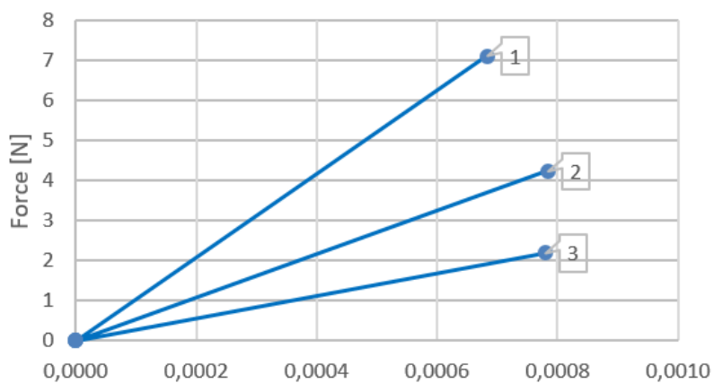
Figure 3 Force-displacement curves of different unit cell models
