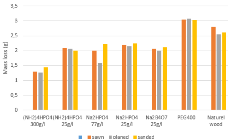
Figure 1 Linder test.
