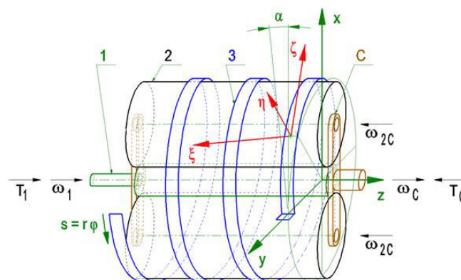
Figure 4 Modelling of the special epicyclic traction drive
