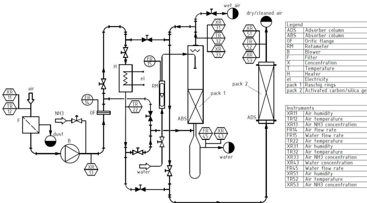
Figure 1 Piping and instrumentation diagram of the test facility
