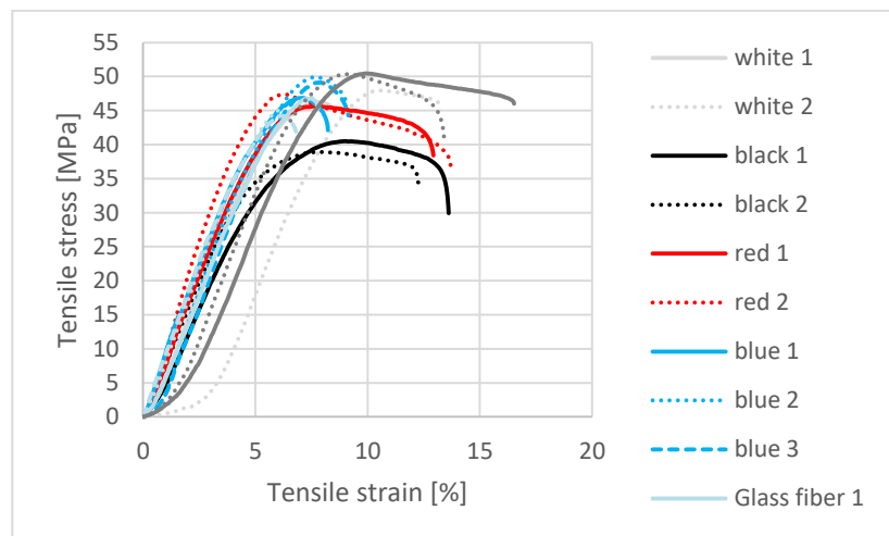
Figure 1 Tensile test: results of all filaments
