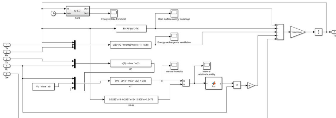
Figure 2 Barn model
