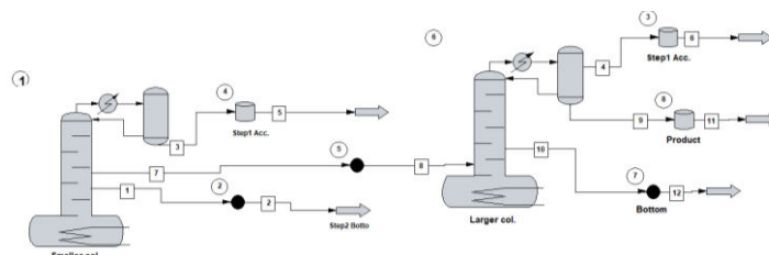
Figure 1 ChemCAD flowsheet of the process
