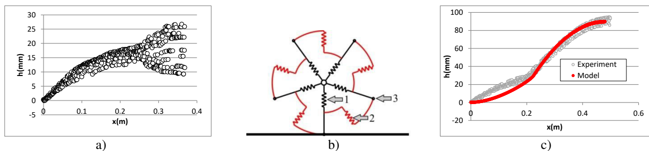
Figure 3 a) Unambiguous results of the response curve obtained experimentally; b) Schematic view of tire model with radial and inter-radial springs used to simulate tire behavior; c) Comparison between model prediction and experimental results
