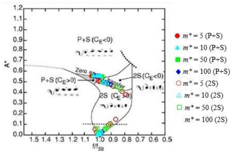
Figure 2 Free vibration points imposed on wake mode map for forced vibration data of Leontini et al [5]
