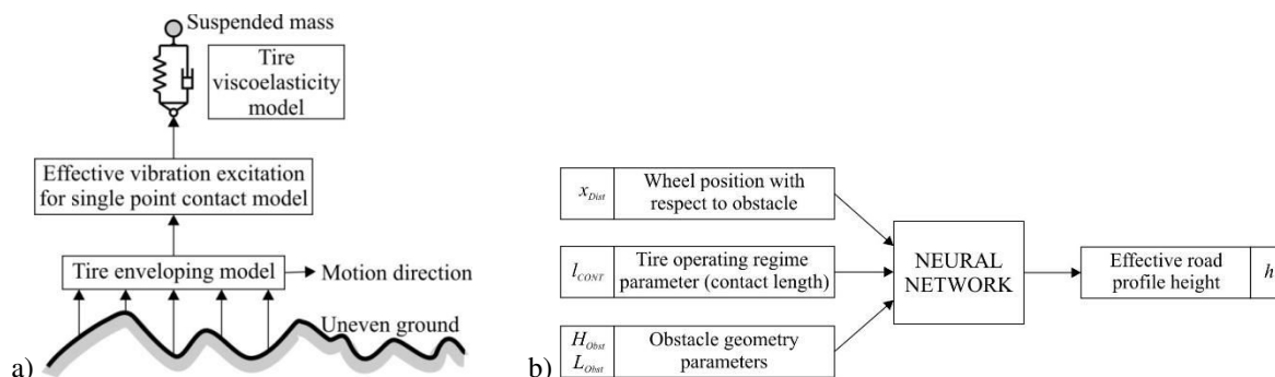
Figure 2 a) Schematic view of separation of the tire model into parts responsible for road profile filtering and for tire viscoelasticity; b) Structure of NN based empirical model of tire enveloping behavior for rectangular shaped obstacle
