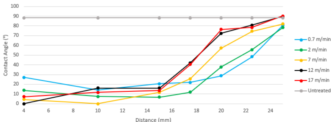
Figure 2 Measured contact angles of the treated samples with water
