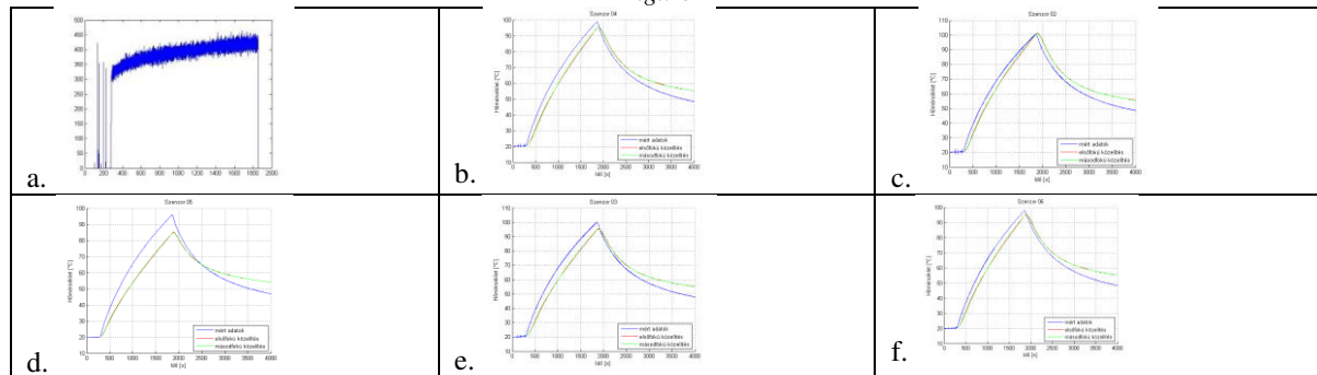
Figure 3 Comparison of the FE simulated and measured temperature variation at different position of PM motor.
