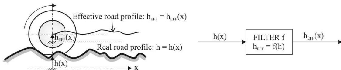
Figure 1 Tire as geometric low-pass filter for road undulations
