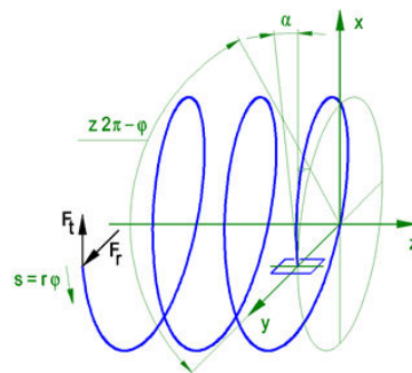
Figure 3 Modelling of the special helical torsion spring
