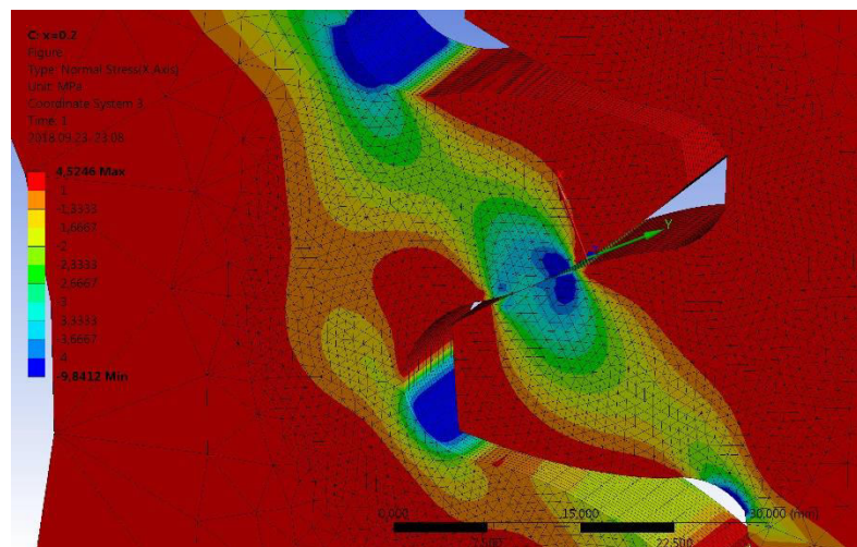
a) The distribution of the normal stress on the connecting surfaces
