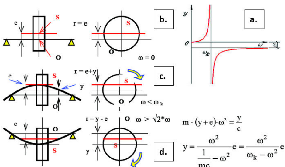
Figure 2 The critical speed of the rotor
