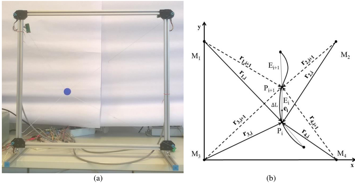
Figure 1. a/ Structure of the cable robot, the end-effector is represented by a blue disk b/ Path of the end-effector
