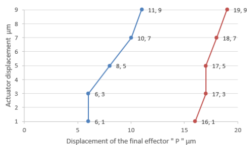
Figure 5a Circular joint profile
