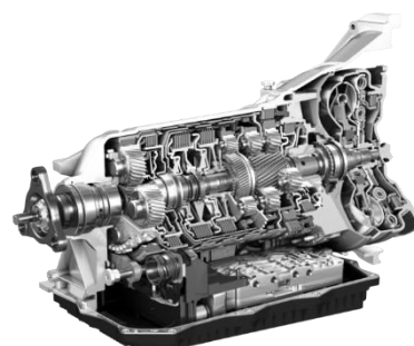
The new product: ZF 8HP transmission
