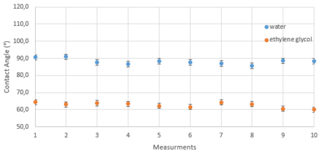
Figure 1 Contact angles on the untreated samples
