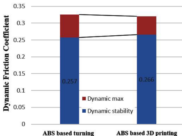
Figure 3 Measurement data of the dynamic friction coefficient
