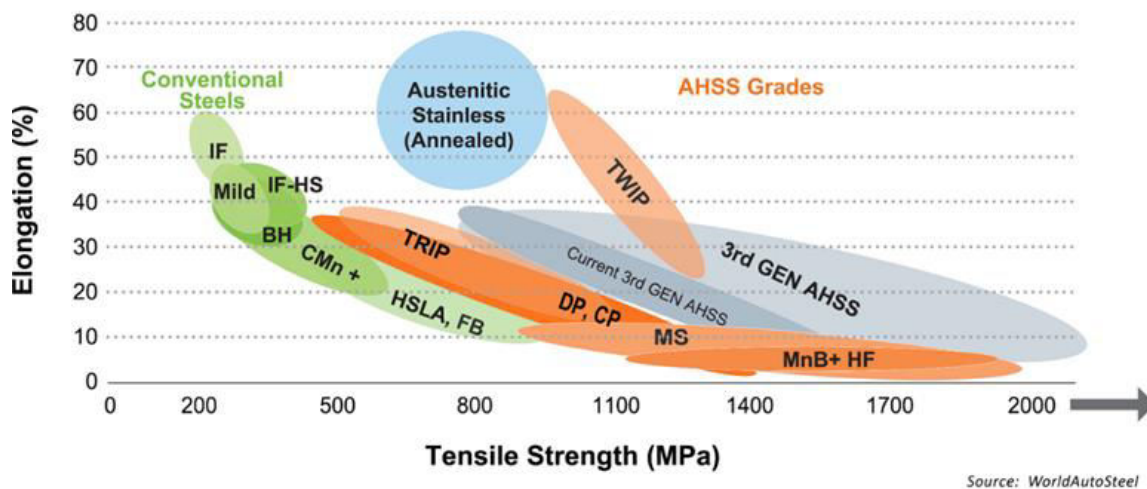
Figure 2 Steel Strength Ductility Diagram, illustrating the range of properties available from today's AHSS grades
