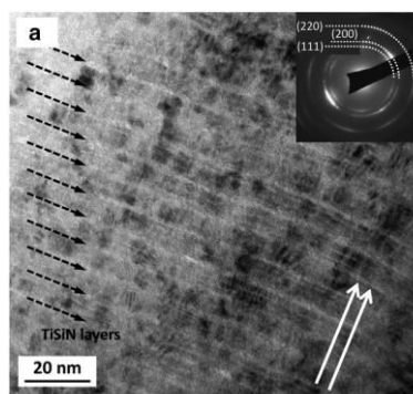
Figure. 3 TEM micrographs of TiAlSiN coating (image with the electron diffraction pattern)
