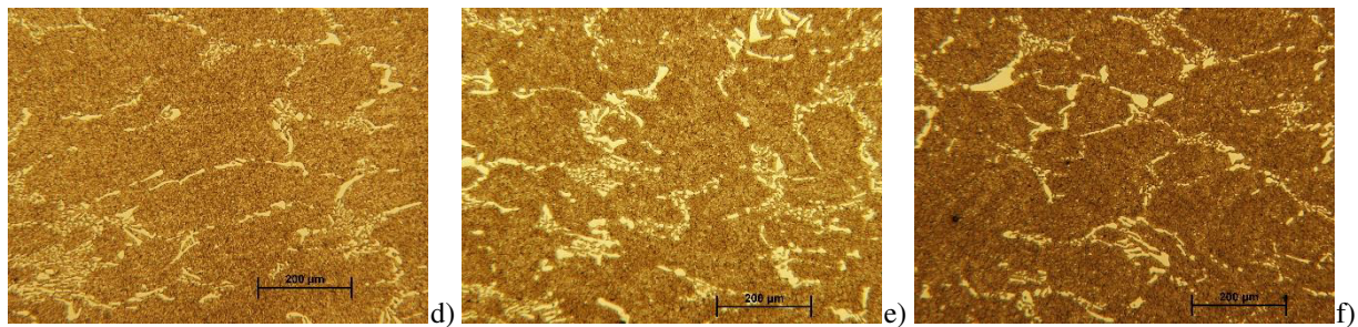
Figure 1 The appearance of primary carbide net a) delivery condition, (b) quenched to RT and tempered at 200°C, (c) quenched and tempered at 510°C (d) quenched and triple tempered ( 510°C+480°C+480°C), (e) quenched, cryrogenically treated and tempered at 510°C (e) quenched, cryrogenically treated and triple tempered (510°C+480°C+480°C). N_{original}=100x . Nital 2%.
