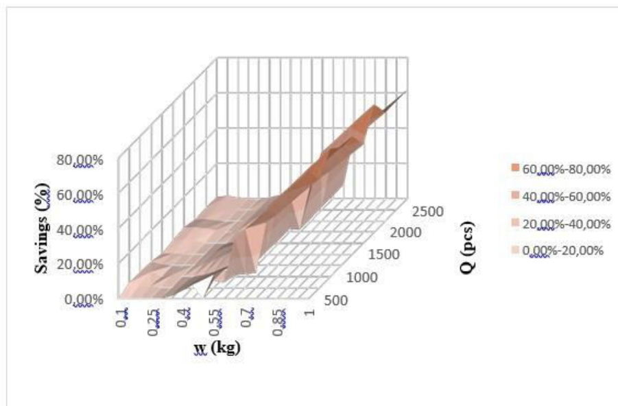
Figure 1 Savings of the model with d1=3 m and d2=20 m
