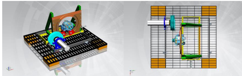
Figure 3 3D assembly model of the final MDDT
