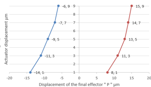
Figure 5b Elliptical joint profile
