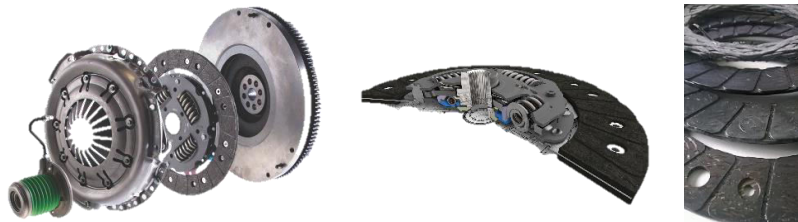
Figure 1 From left to right: Parts of a dry clutch system, dry clutch plate, products of phases of dry friction material production [1]
