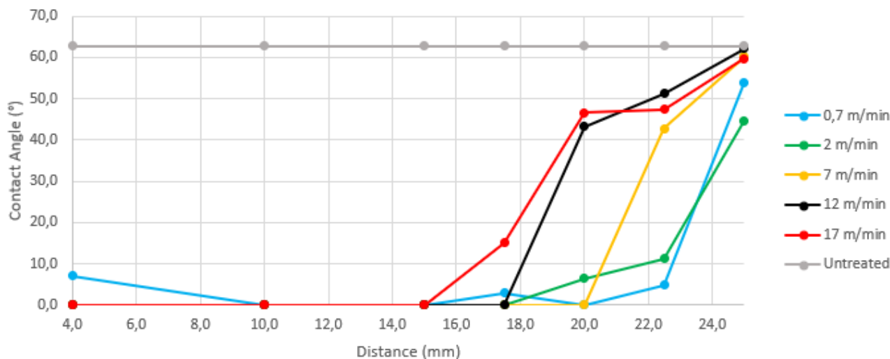
Figure 3 Measured contact angles of the treated samples with ethylene glycol
