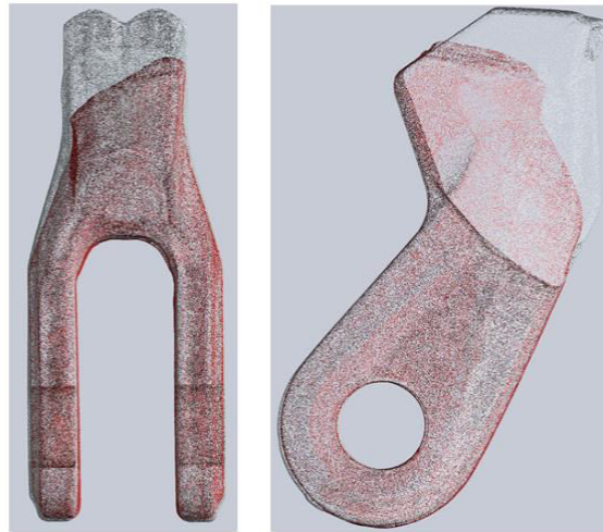
Figure 2 Loss of material displayed on the tool
