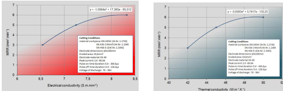
Figure 3 Dependence of MRR on electrical and thermal conductivity of machined material for EDM of tool steels with graphite electrode EX-60
