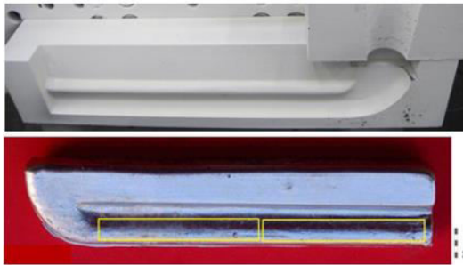
Figure 2 Diez-test die and the locations of the tensile specimens
