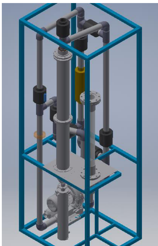
Figure 2 The 3D model and setup interval of the test facility
