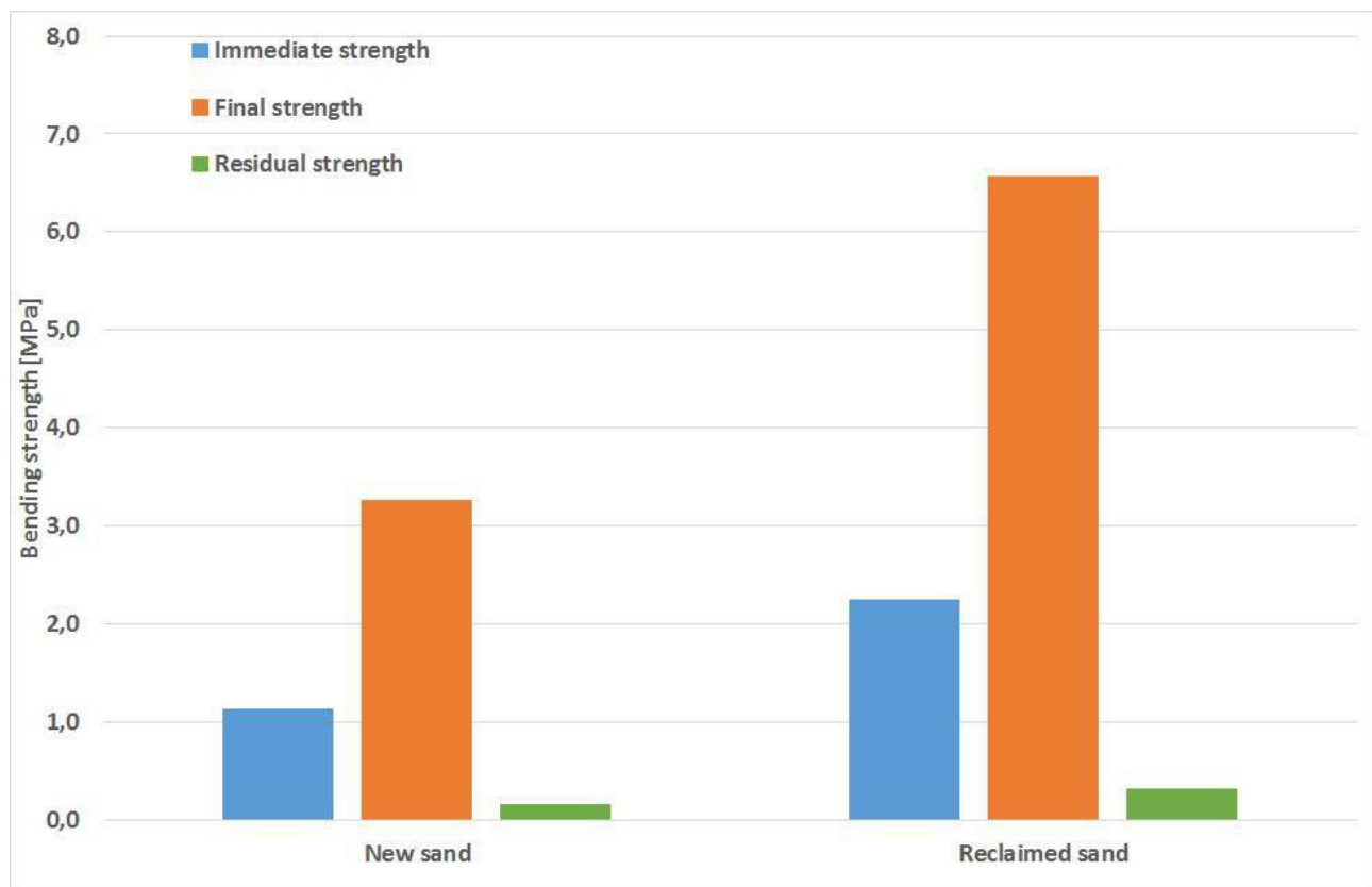
Figure 1 Bending strength of new sand and mechanically reclaimed sand
