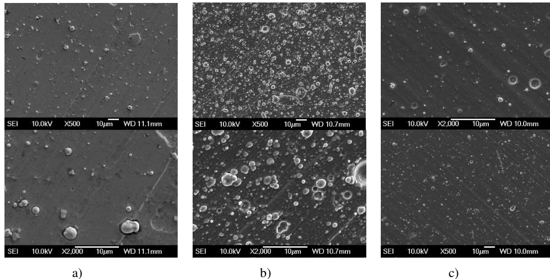
Figure 3 Surfaces of: a) ZrN, b) TiCN MP and c) CrN coatings
