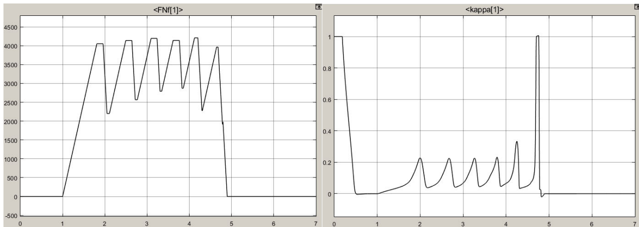
Figure 1 Brake force resulted by an ABS controller and the corresponding slip
