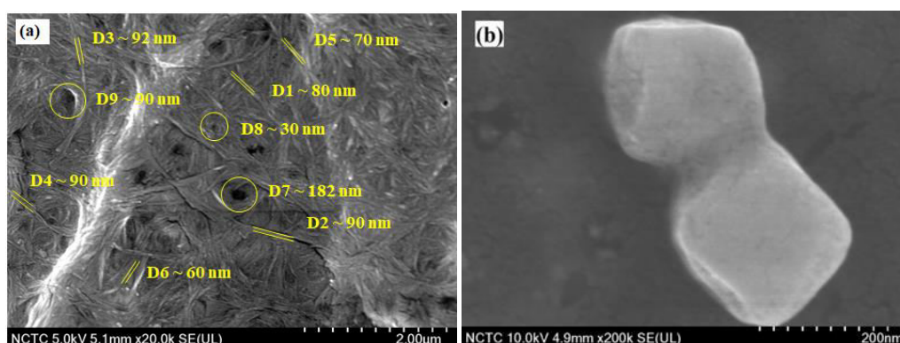
Figure 1 FE-SEM micrographs of a) BS-SF-PVA film, b) silver nanocubes.
