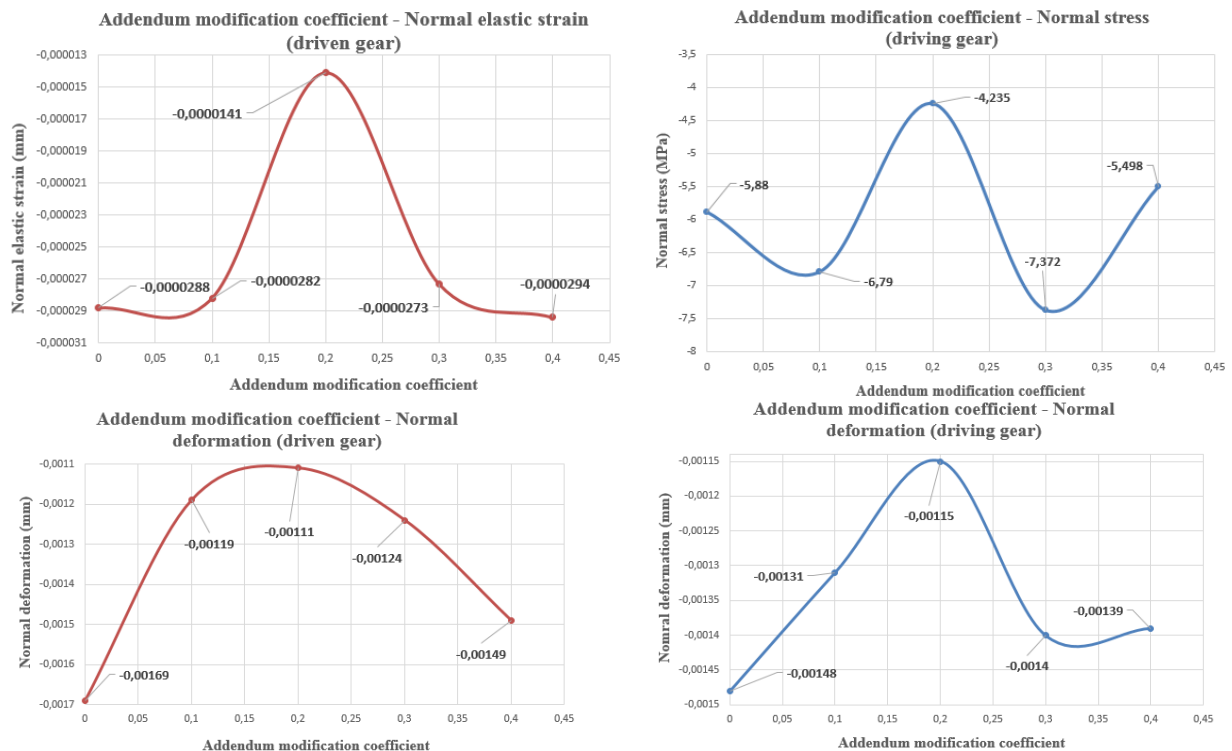
Figure 3 The analysed TCA parameters in the function of the addendum modification coefficient
