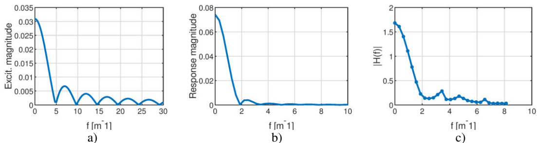
Figure 4 a) Magnitude of the input spectrum; b) Magnitude of the output spectrum; c) Averaged frequency response function magnitude
