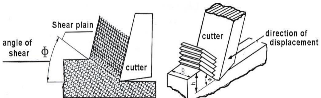
Figure 1 Process of cutting (the inside friction)
