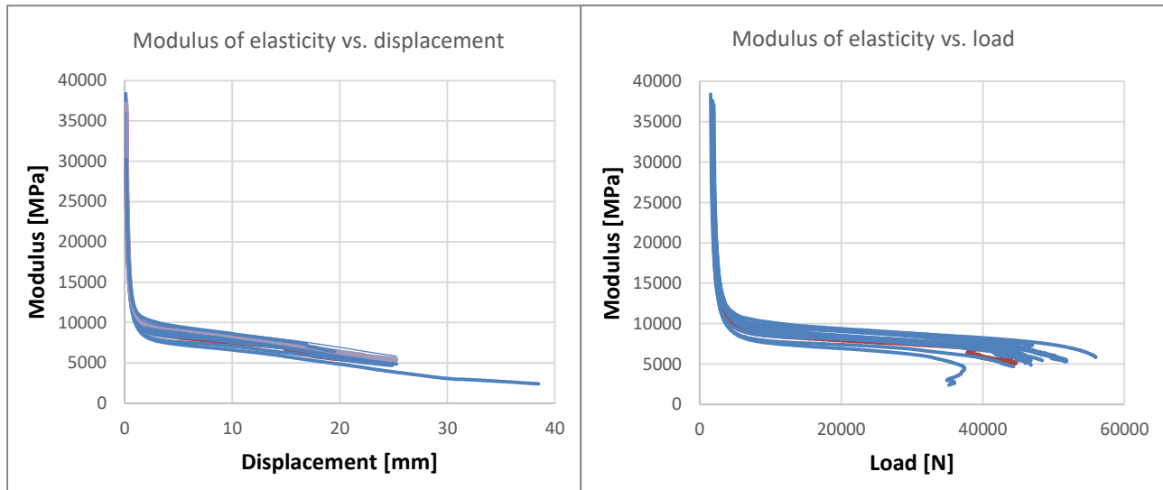
Figure 2 Modulus of elasticity of reinforced beams vs. mid-span displacement and load
