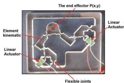
Figure 1 Pentalater mechanism
