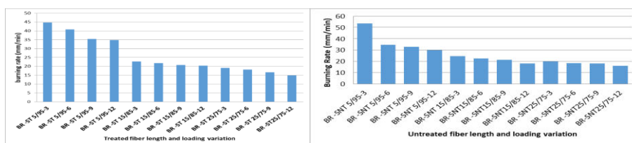
Figure 1 Effect of treatment, fiber length and fiber loading on burning rate of SFRPP composite
