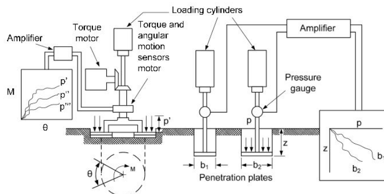
Figure 1 Schematic diagram of a Bevameter
