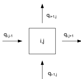
Figure 2 Heat fluxes for cell i,j
