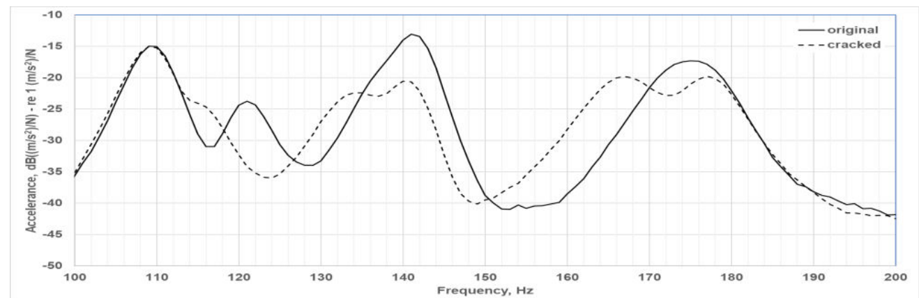
Figure 4 The average of the measured FRFs for the uncracked and for the cracked specimen from 100 to 200 Hz.
