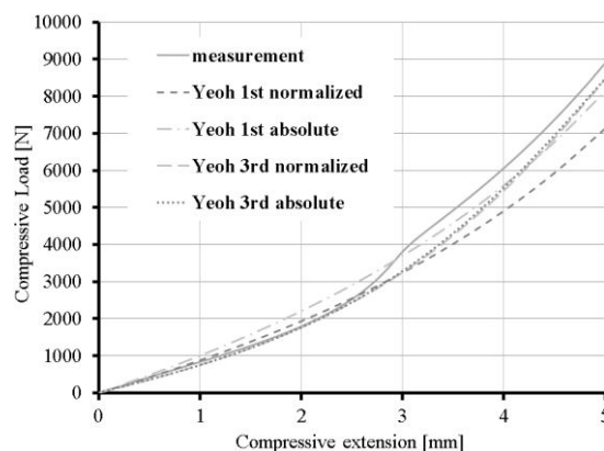
Figure 2 Finite element results using Yeoh material models
