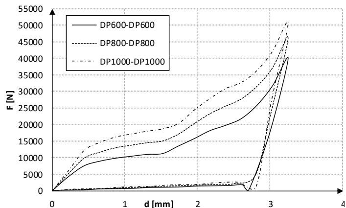
Figure 2 Comparison of the forming force-relative punching tool displacements in case of different steels
