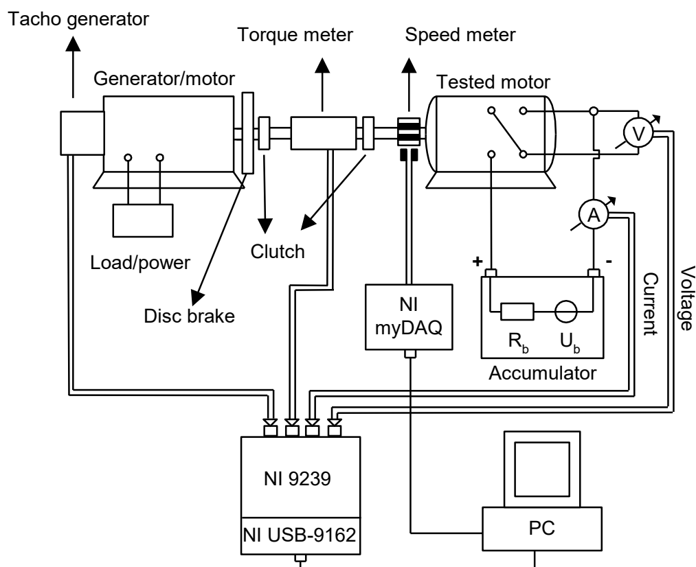
Figure 2 The measurement layout
