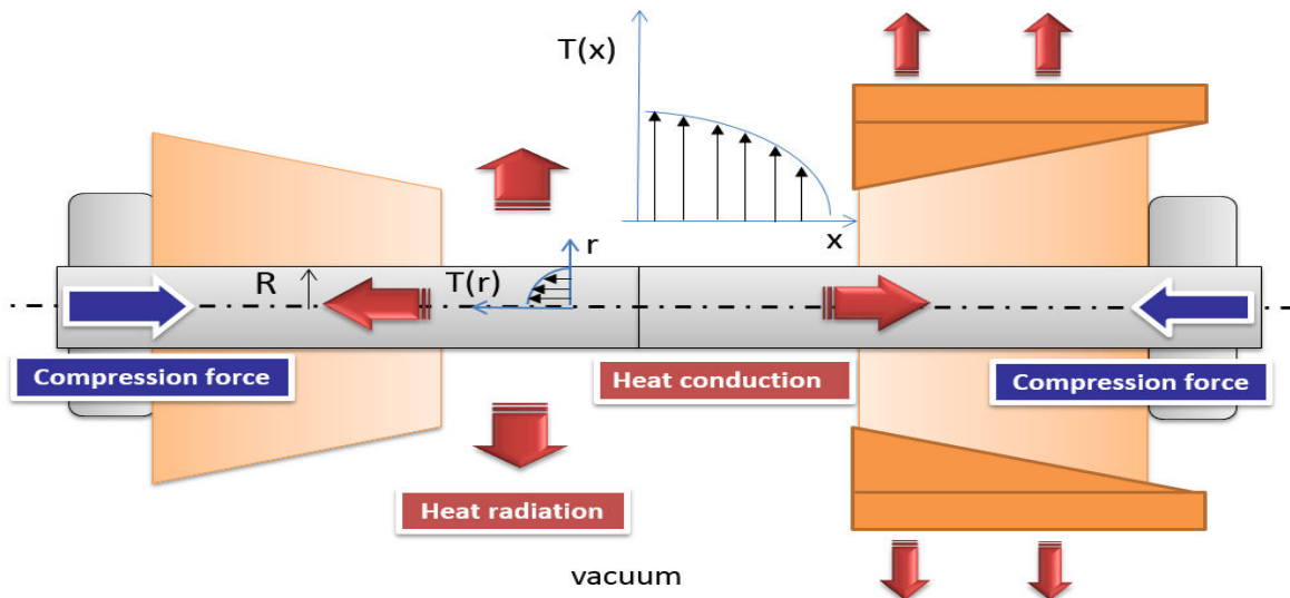
Figure 1 Schematic view of specimens with copper jaws for temperature distribution
