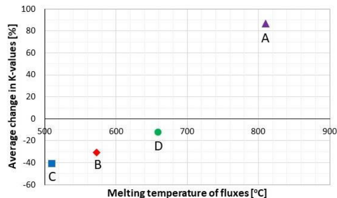
Figure 2 The comparison of melt cleaning efficiency and the melting temperature of fluxes
