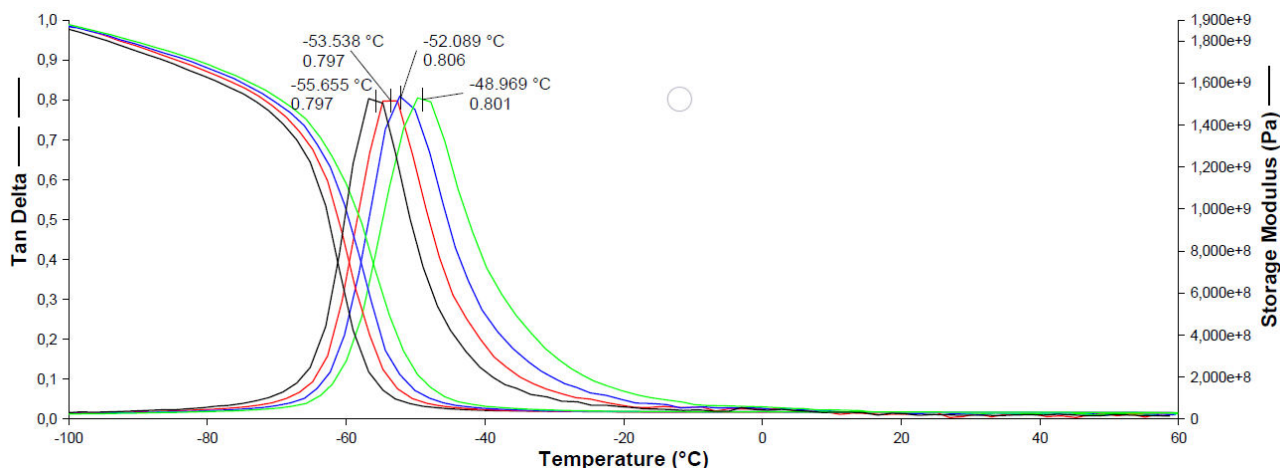
Figure 3 DMTA curves of Coconut oil mixed sample on different frequencies: 0,3; 1,0; 3,0 and 10,0 Hz
