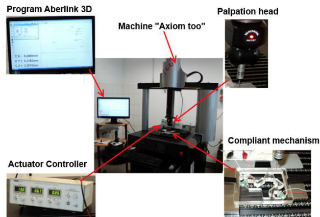
Figure 4 Experimental stand
