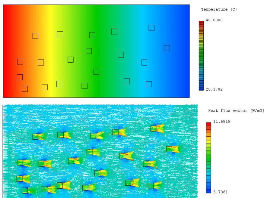
Figure 4 Temperature distribution and heat flux vectors. (Cedar wood used as biomass and Polystyrene used as base material)
