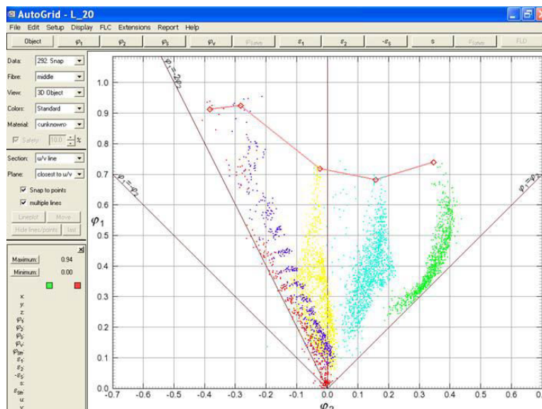
Figure 3 Graphical generation of FLC from the measured strains.
