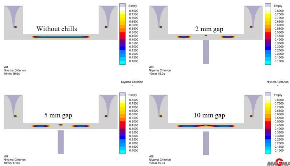
Figure 3 Simulated Niyama criterion values for drag chills that create end zone effect between two feeders
