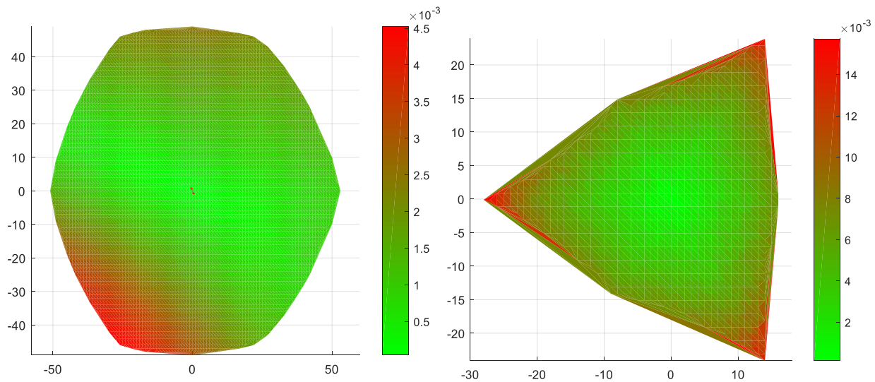
Figure 2 Error visualization for the general type (left) and rotary type (right) Stewart platforms
