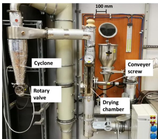
Figure 1 Photo of the fluidized bed dryer
