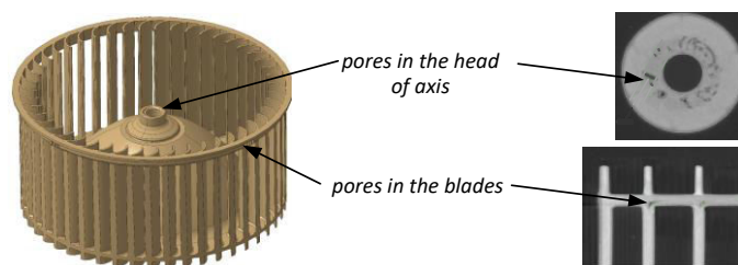
Figure 1 Material defects in the injection-moulded impeller
