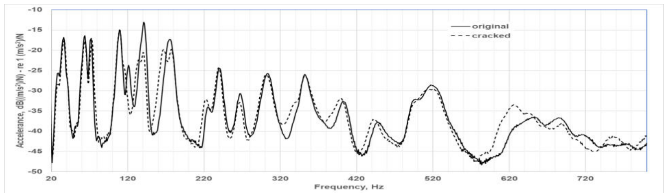
Figure 3 The average of the measured FRFs for the uncracked and for the cracked specimen.
