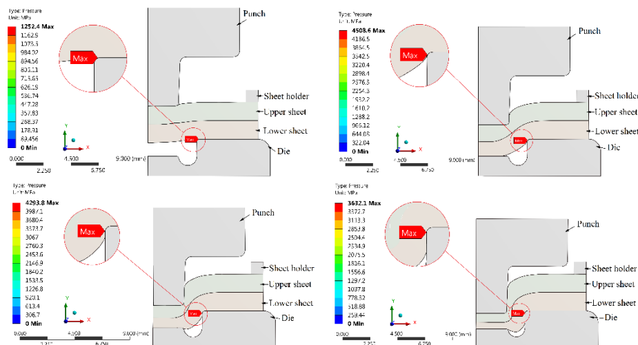
Figure 2 Clinching process: a) max. contact pressure during drawing, b) max. contact pressure during compression, c) max. contact pressure during interlocking, d) max. contact pressure during backward extrusion
