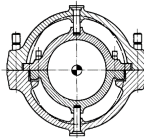
Figure 2 The connection between casings allows different thermal expansions for the outer and inner casing
