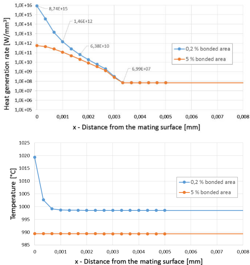
Figure 3 Heat generation rate and temperature distribution in specimen near to the joining surface in contact asperities in steady state
