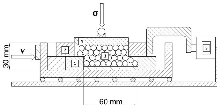
Figure 1 Schematic design of the direct shear box apparatus (1 - Lower shear box, 2 - Upper shear box, 3 - Granular material, 4 - Load plate, 5 - Load cell, \sigma - Normal stress, v - Shear velocity) [5]
