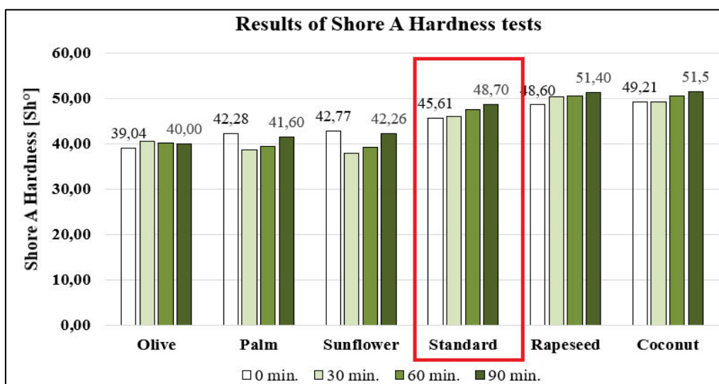
Figure 2 The results of Shore A Hardness tests
