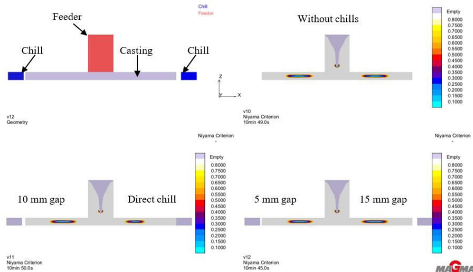
Figure 2 Simulated Niyama criterion values for end chills that increase end zone length
