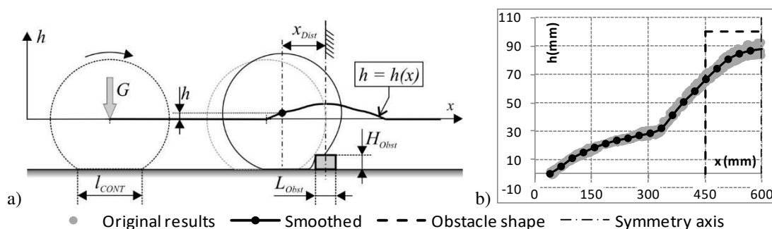
Figure 1 a) Example of the tire enveloping curve for the singular ground obstacle of rectangular cross section: h - effective road profile height, x - longitudinal wheel travel, h=h(x) - enveloping curve, G - vertical force exerted at the wheel, l_{CONT} - tire contact length on the level ground, x_{Dist} - wheel position with respect to the obstacle, L_{Obst} , H_{Obst} - obstacle dimensions; b) Graphical representations of typical test results (only first half of input and output curve shown, i.e. up to the vertical axis of symmetry)
