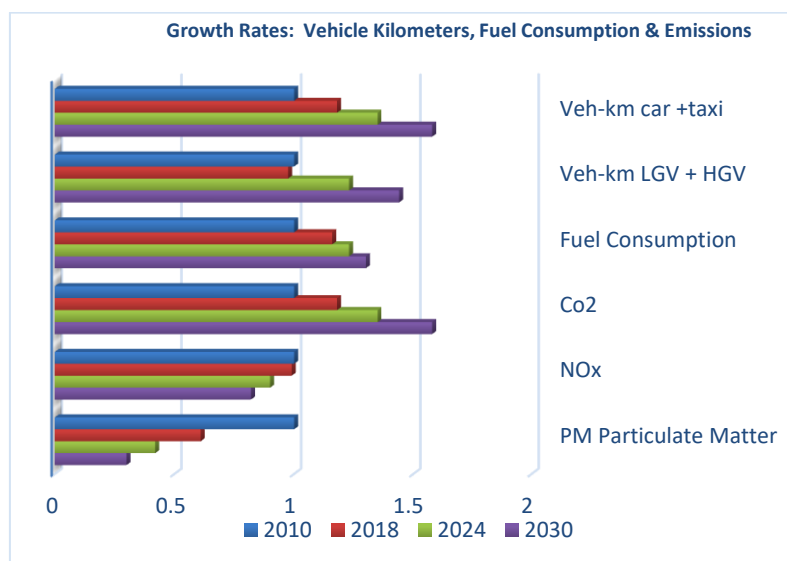
Figure 1 Growth Rate: Vehicle kilometers, Fuel Consumption and Emissions
