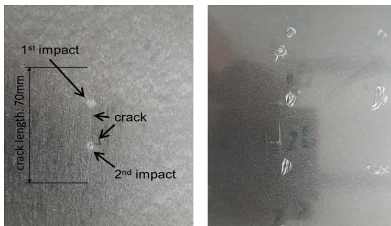
Figure 2 Damage of the specimen (left: side of the impact; right: back side)
