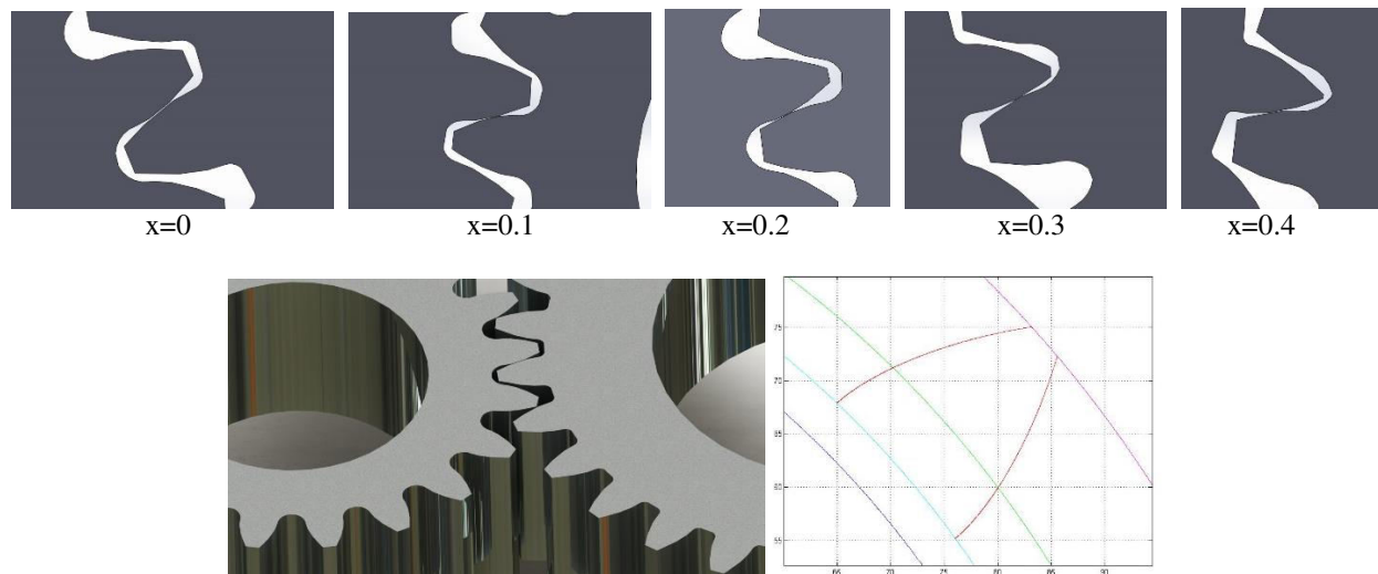
Figure 1 Designing of the spur gears having different addendum modification coefficients
