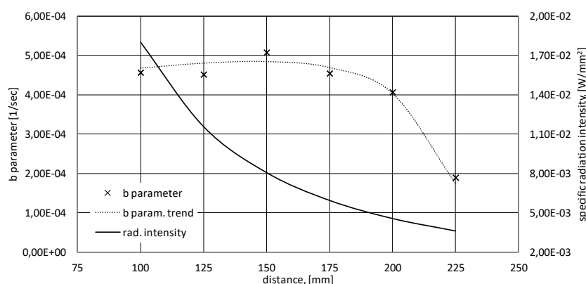
Figure 1 Parameter b of H-P model and radiation intensity in function of tomato – bulb distance
