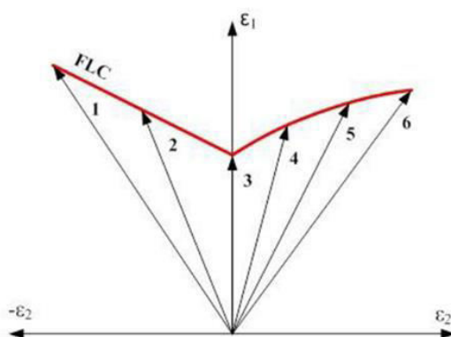
Figure 1 Forming Limit Diagram for various strain paths (1-pure shear, 2-uniaxial tension; 3-plain strain; 4, 5 6-different biaxial tension)
