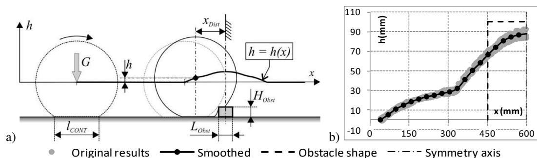
Figure 2 a) Example of the tire enveloping curve for the singular ground obstacle of rectangular cross section: h - effective road profile height, x - longitudinal wheel travel, h=h(x) - enveloping curve, G - vertical force exerted at the wheel, l_{CONT} - tire contact length on the level ground, x_{Dist} - wheel position with respect to the obstacle, L_{Obst} , H_{Obst} - obstacle dimensions; b) Graphical representations of typical test results (only first half of input and output curve shown, i.e. up to the vertical axis of symmetry)
