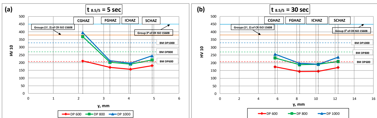
Figure 2 Hardness of simulated HAZ (a) t_{8.5/5} = 5 s and (b) t_{8.5/5} = 30 s
