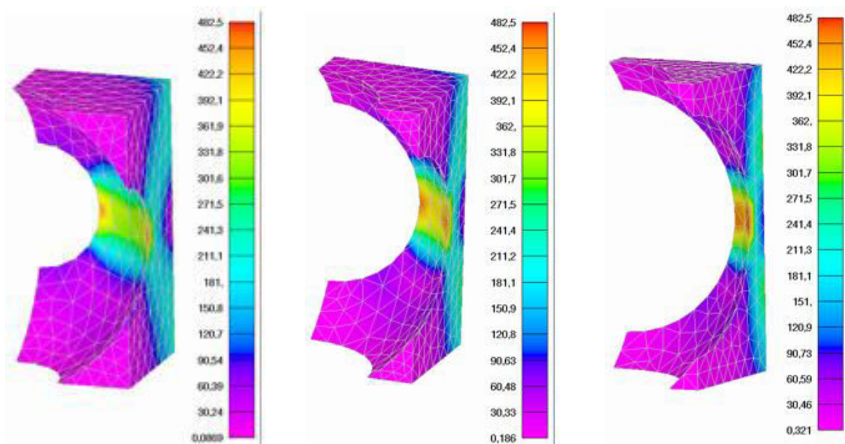
Figure 2 FEA results of the unit cell models
