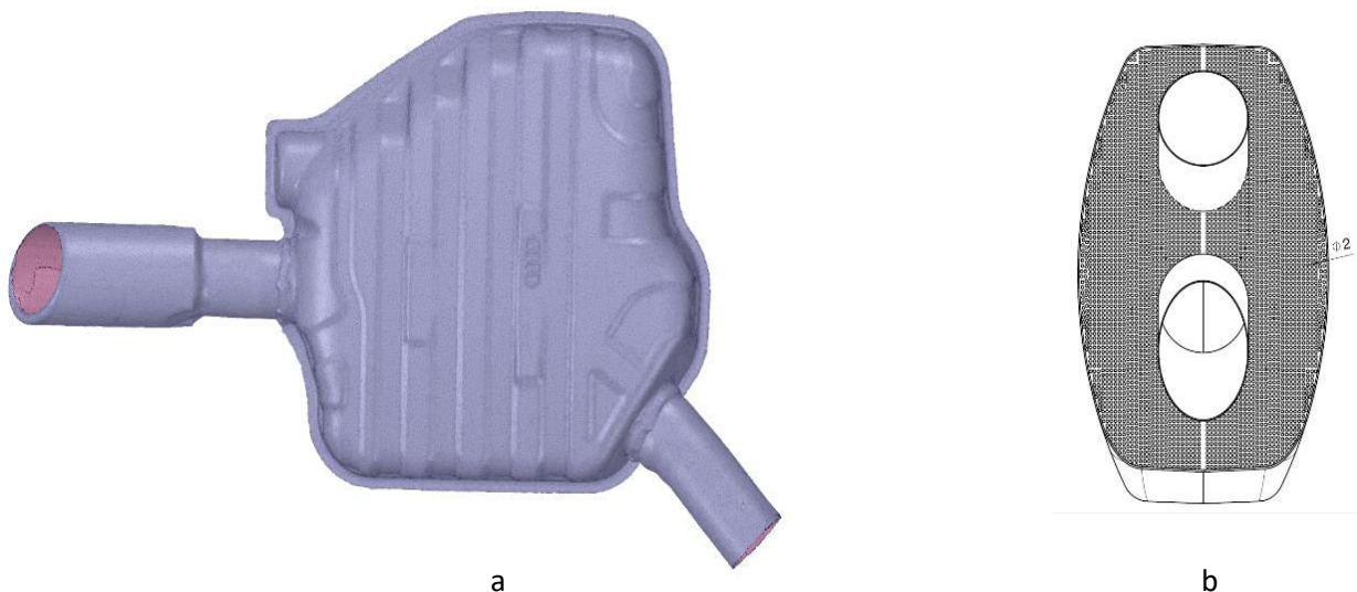
Figure 1 (a) Muffler geometry, (b) porous plate part inside the muffler
