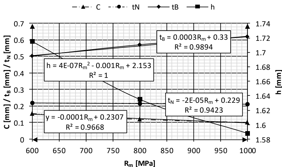
Figure 4 Relationship between the UTS and geometrical properties
