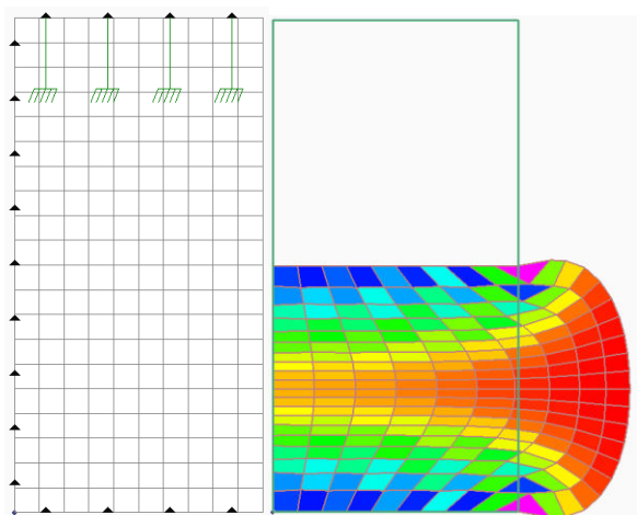
Figure 3 Deformation state of a rubber bumper with the use of quadrilateral elements for meshing
