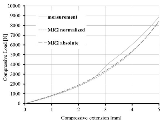
Figure 1 Finite element results using two-term Mooney-Rivlin material models
