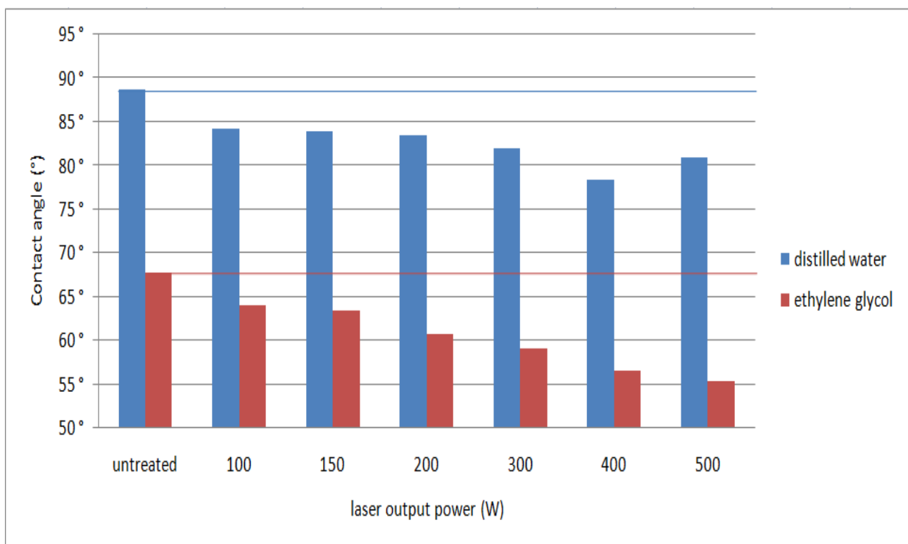
Figure 1 Distilled water and ethylene glycol contact angles on laser treated surface
