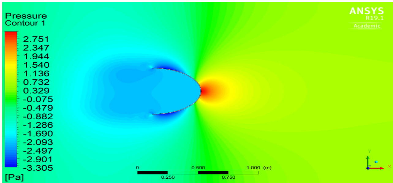
Figure 2 pressure distribution around the surface of the blade
