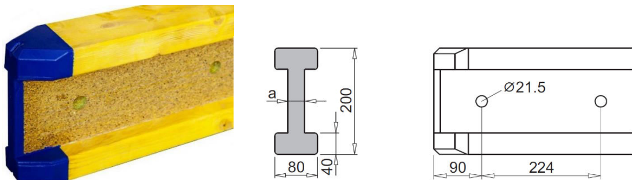
Figure 1 Formwork beam and specifications
