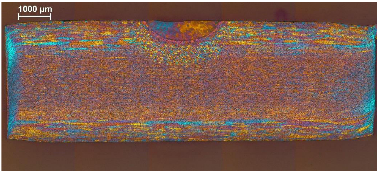
Figure 1 Microstructure of the LASER treated aluminium sheet.
