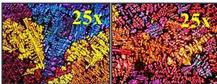
Figure 1 The Barker colour etched micrographs: (a) 3 rd alloy before grain refinement, (b) after the addition of AlTi5B1 grain refining master alloy
