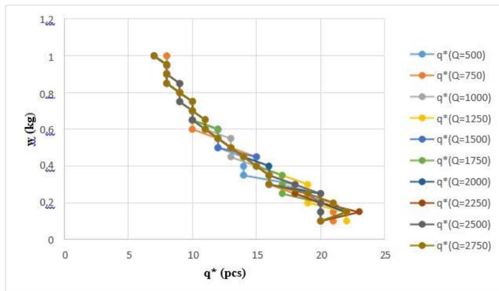
Figure 3 Optimal lot-size for different total amount of handled item and unit weight of item ( d1=3 m and d2=20 m)
