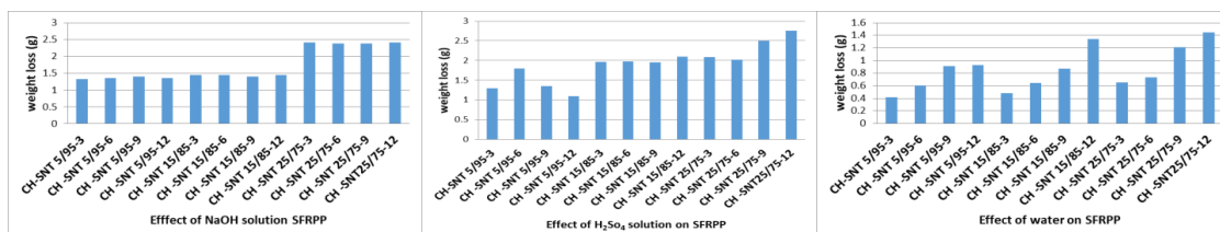
Figure 2 Effect of fiber length and fiber loading on chemical resistance of untreated SFRPP
