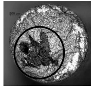
Figure 3 The stereo microscopic image of a chosen test bar
