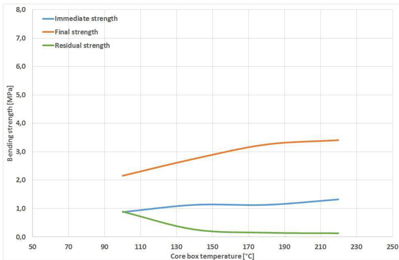
Figure 2 Bending strength of new sand and mechanically reclaimed sand
