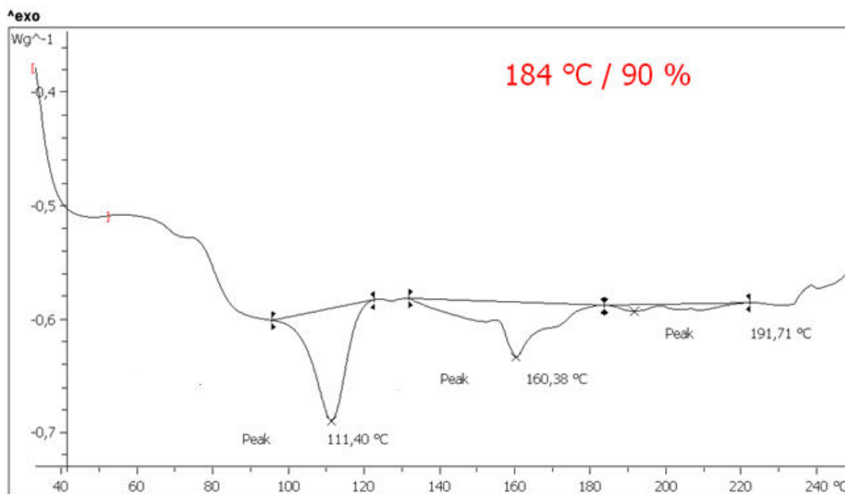
Figure 2 DSC curve of PVC/LDPE foam blend
