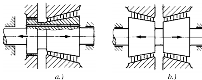
Figure 3 Balancing of the axial forces with a.) dummy-disc and with b.) double-flow structure
