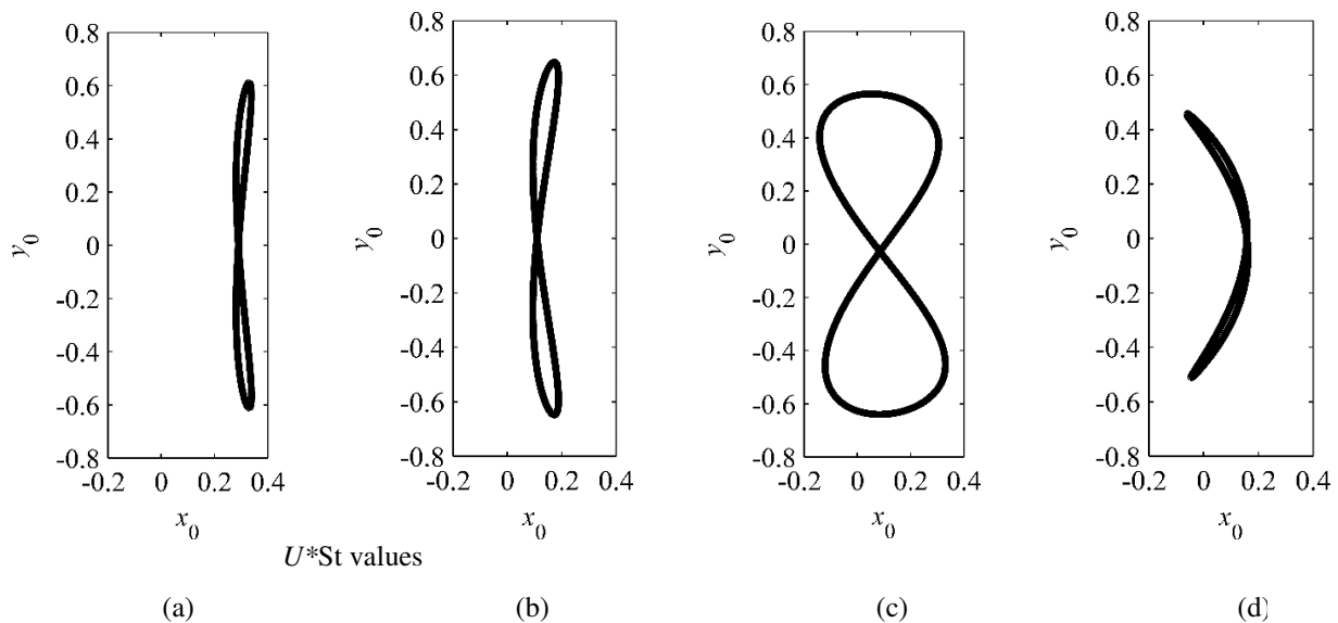
Figure 2 Cylinder path at FR=1 (a), 1.5 (b), 2.0 (c) and 2.5 (d) for U^*St = 0.9
