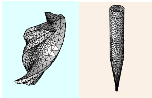
Figure 1 Meshed model of the micro-cutting tools
