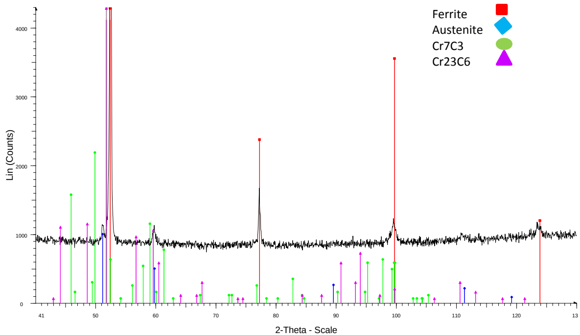
Fig.9.Full XRD spectra of samples H12_2a
