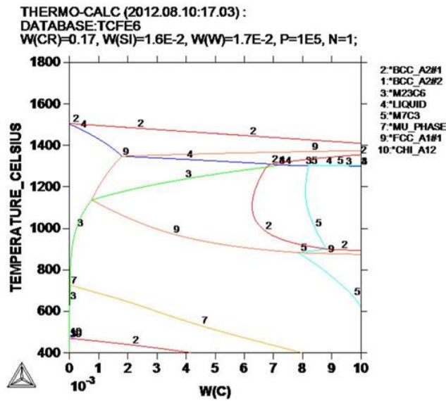
Fig.2. The calculated phase equilibrium diagram for the Fe, Cr, Si, W and C constitutions (Thermo-calc), and the half part of casted samples prepared for metallographic investigation
