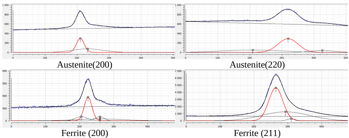
Fig.10. XRD spectra of samples H12_3 determined by position sensitive detectors
