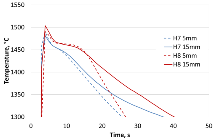
Fig. 3. The recorded cooling curves at the 5 mm and at the 10 mm section of samples H7 and H8
