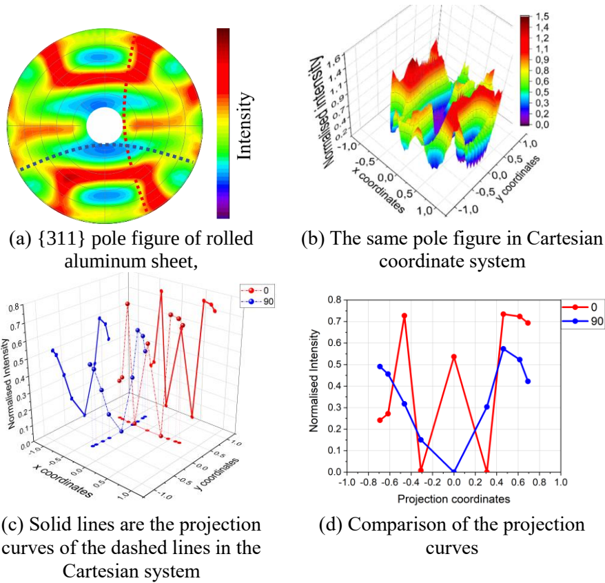
Figure 1. Procedure for qualitative texture description [13]. Dashed lines represent data obtained from stress measurements.
