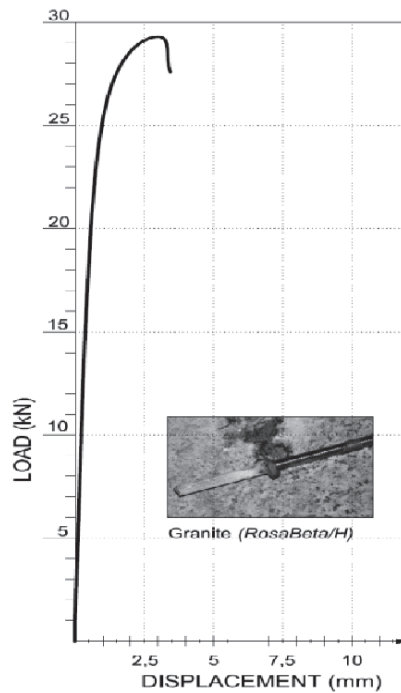
Figure 10. Pull-out failure curve
