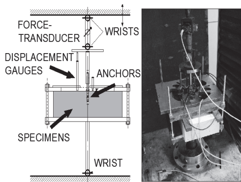
Figure 7. Arrangement of pull-out tests.
