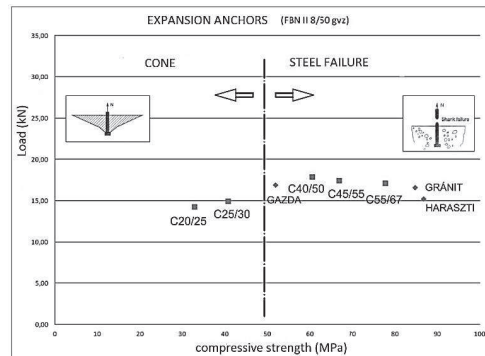
Figure 12. Critical force - Compressive strength of concrete and stone
