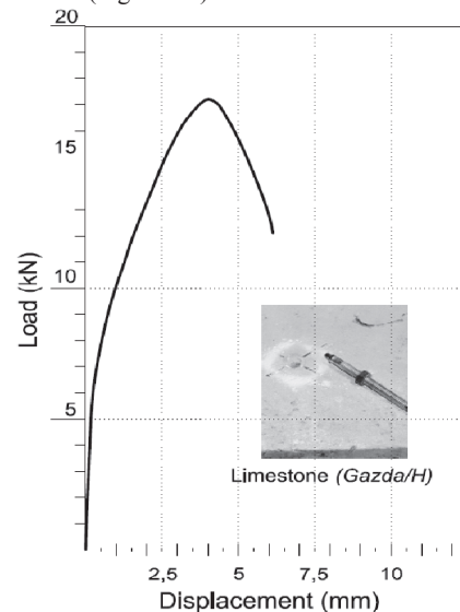
Figure 8. Typical steel failure curve
