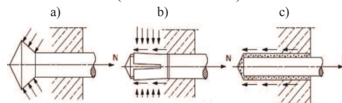
Figure 1. Load transfer methods: mechanical interlock (a), friction (b), bonding (c)
