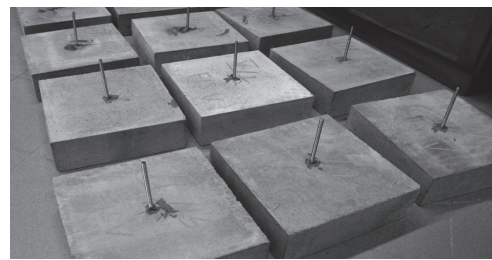
Figure 5. Concrete specimens for pull-out tests
