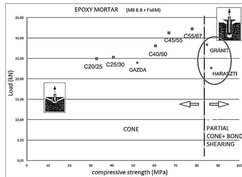
Figure 13. Critical force - Compressive strength of concrete and stone
