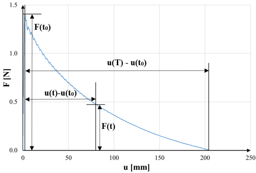
Figure 3 Yarn pull-out diagram of a typical glass woven fabric, with force and displacement type quantities from Equation (1)
