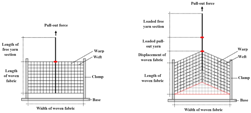
Figure 1 Principle of yarn pull-out
