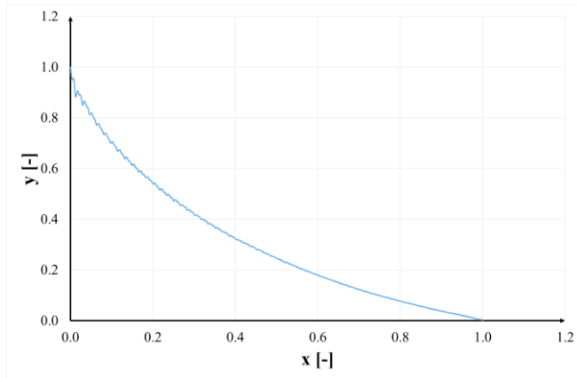
Figure 9 UTE 195P basis curve
