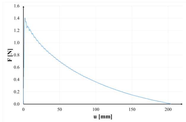
Figure 8 UTE 195P mean curve
