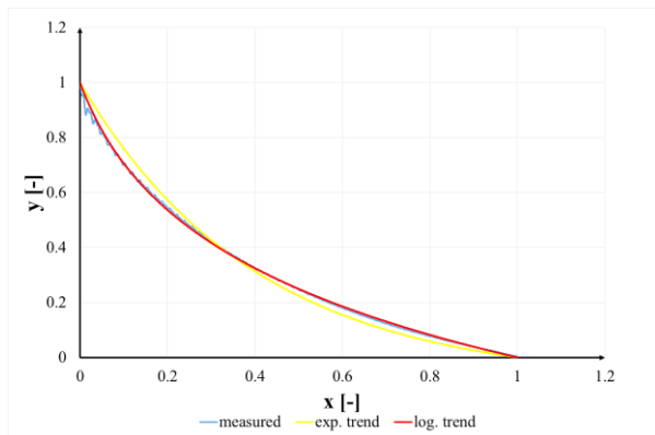
Figure 11 Fitting an exponential and a logarithmic trend to the UTE 195P basis curve
