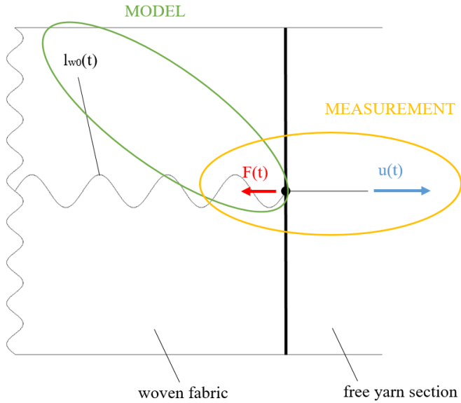
Figure 2 Conceptions of the yarn pull-out cases
