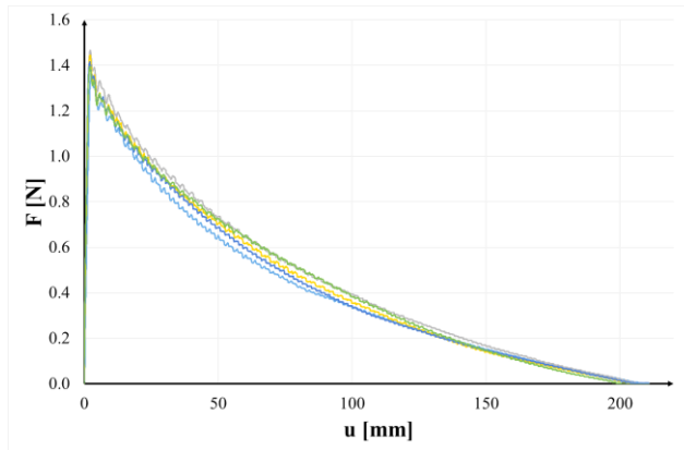
Figure 7 UTE 195P yarn pull-out curves
