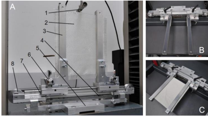
Figure 5 Multifunctional woven fabric testing device
