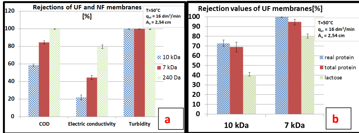
Fig. 4. Rejection values measured calculated for different UF and NF membranes:
