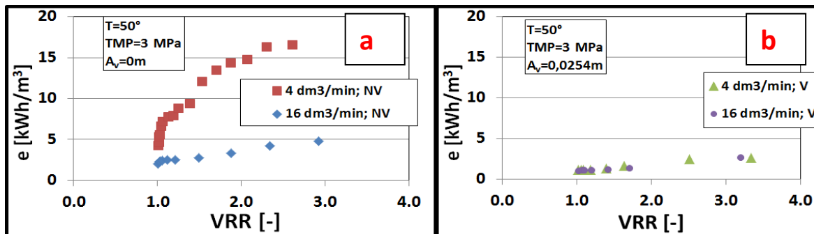
Fig. 2. Specific energy demands in low and high recirculation flow rate experiments: (a) non-vibration mode, (b) vibration mode
