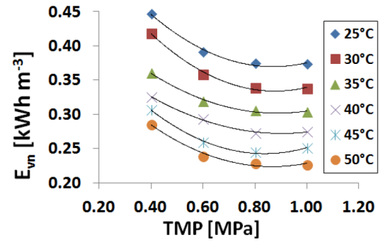
Fig. 2. The effect of water temperature on the non-vibration specific energy consumption (Ultrafiltration; A_v = 0 ; q_{vrec} = 16 \text{ dm}^3 \text{min}^{-1} ).
