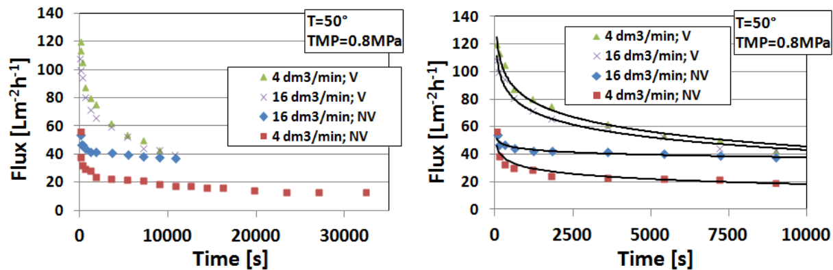
Fig. 3. The effects of recirculation flow rate and module vibration on ultrafiltration fluxes (V: vibration mode, A_v = 2.54 \text{ cm} ; NV: non-vibration mode).
