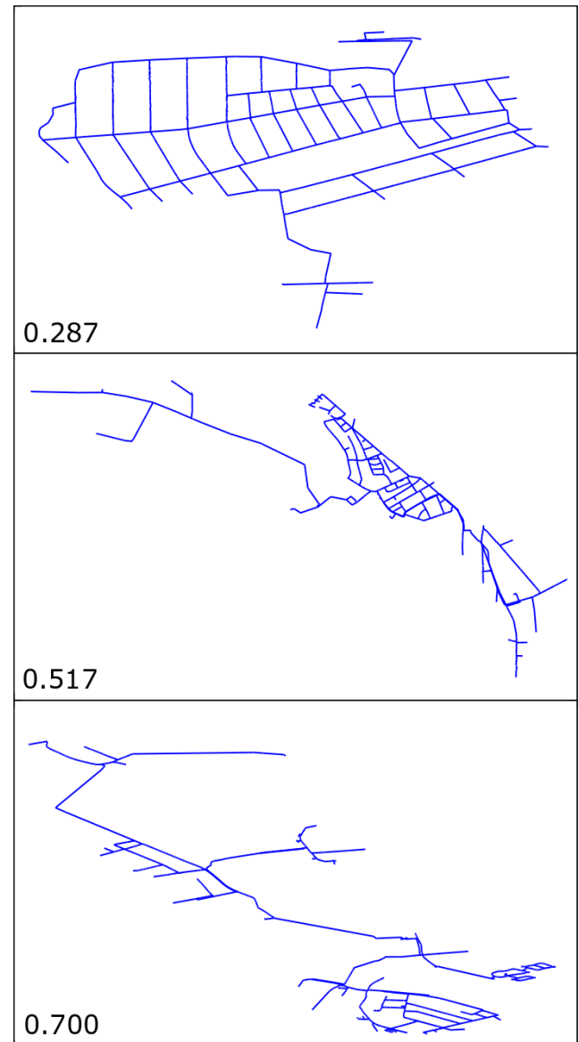
Fig. 7. Visualising different type of network topologies (from urban to suburban side) and indicating the n_{1/3+} on Network 10, 8 and 4.
