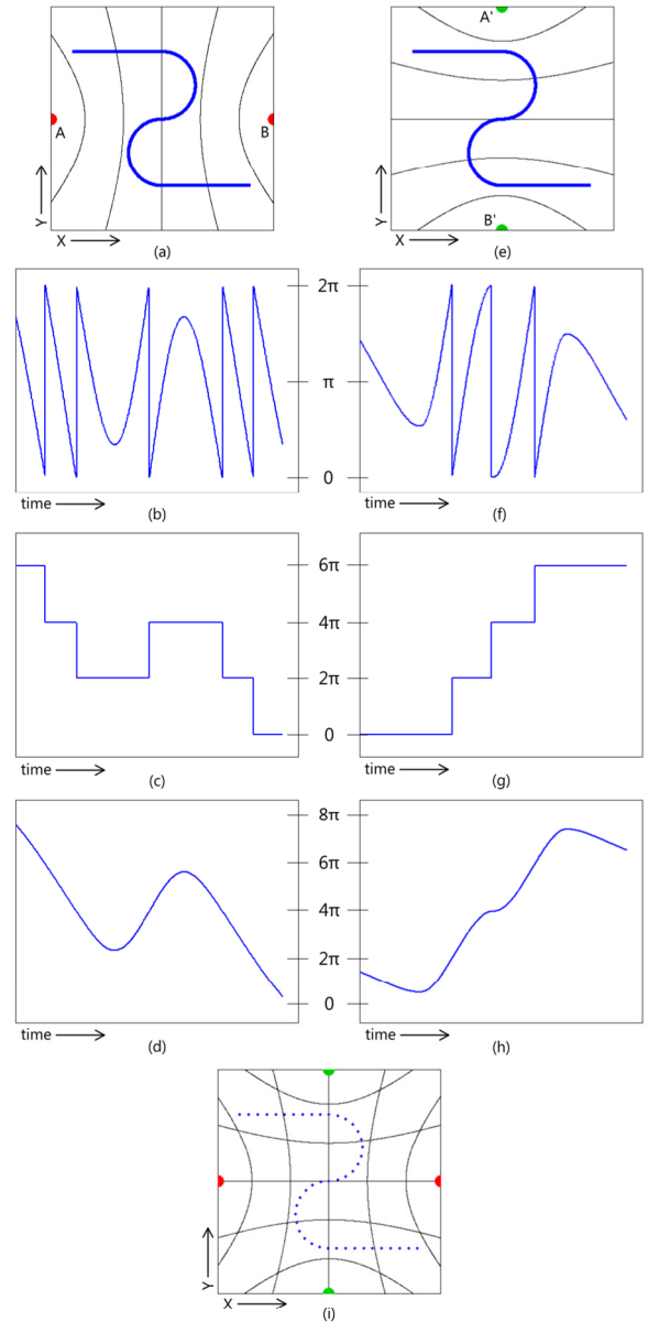
Figure 2. Radio interferometric tracking with fixed transmitters A, B, A', B', fixed receiver C=C', and moving node D. (a) The generated phase pattern by transmitters A and B: hyperbolas corresponding to \vartheta = 2k\pi phase values are shown. The trajectory of the moving object is shown by thick line, the origin is assumed to be known, (b) the measured phase difference values between nodes C and D, (c) phase correction values, (d) unwrapped phase values, (e)-(h) independent measurement with transmitters A' and B', (i) tracking using the phase estimates of the two measurements. The trajectory estimate is shown by the dotted line.
