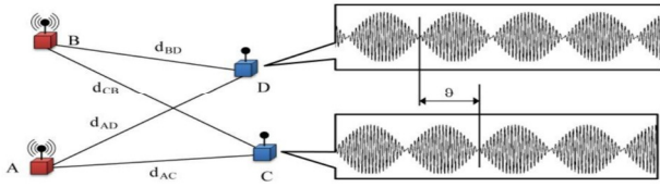
Figure 1. Radio interferometric phase measurement
