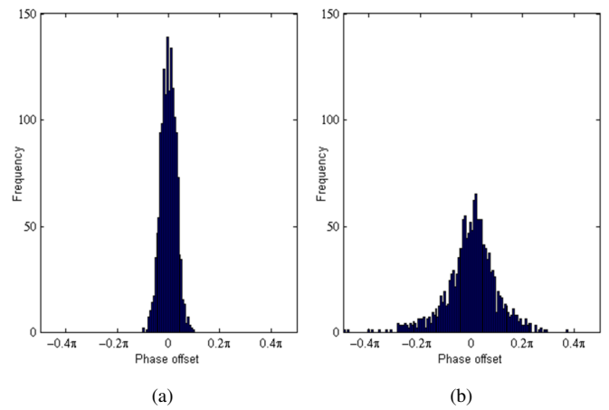
Figure 9. Distribution of 1500 phase offset measurements (a) disturbance-free case (b) human presence and movement
