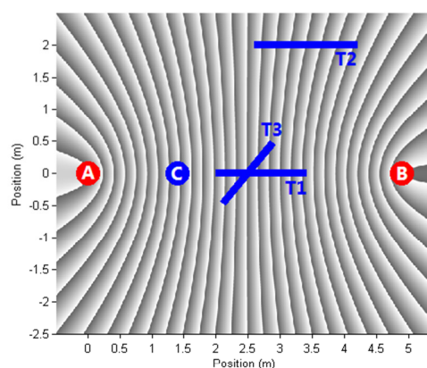
Figure 5. Setup for phase-offset test measurements using fixed transmitters A,B, fixed receiver C, and moving receiver D. Blue line segments show trajectories T1, T2, and T3 of the moving object D. The calculated ideal phase-offset pattern is also shown.
