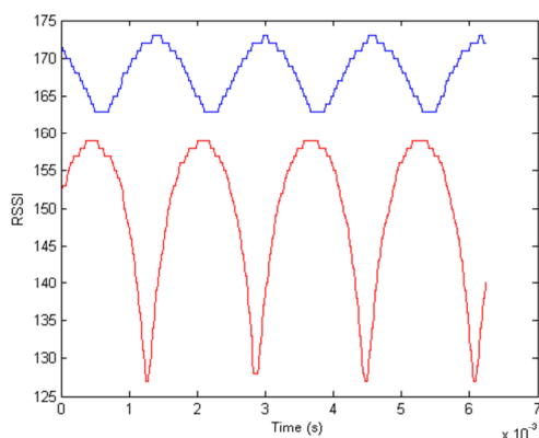
Figure 4. RSSI measurements of an interferometric signal with two synchronized radio receivers (blue and red lines, respectively). The RSSI output of the radio has logarithmic scale.
