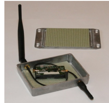
Figure 3. The dual-radio node used in the tests
