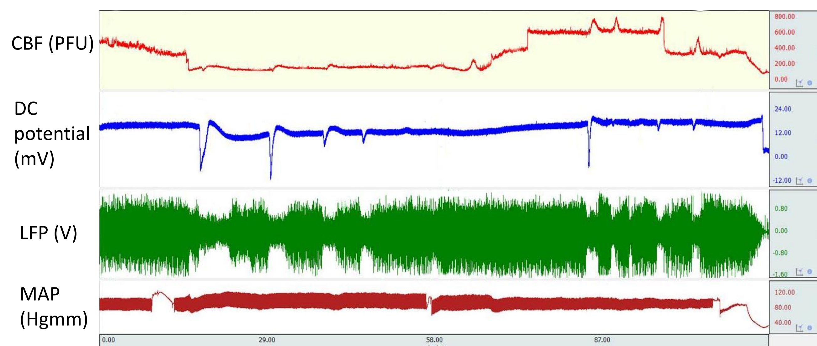
Figure 2. Representative recordings of the four variables under study. 1. Channel (top, red): Laser Doppler Flow (LDF) measured with a stainless steel doppler probe. 2. Channel (blue): DC-ECG was measured via glass microcapillary with differential amplifier in DC-coupled mode. 3. Channel (green): EEG was measured via same glass capillary with differential amplifier in AC-coupled mode. 4. Channel (bottom, drone): MAP was measured via a left femoral arterial catheter.
