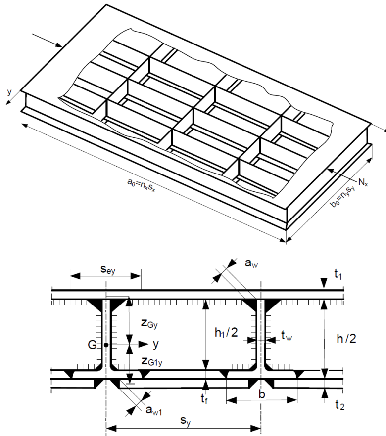
Figure 4. Orthogonally stiffened cellular plate and its cross-section
